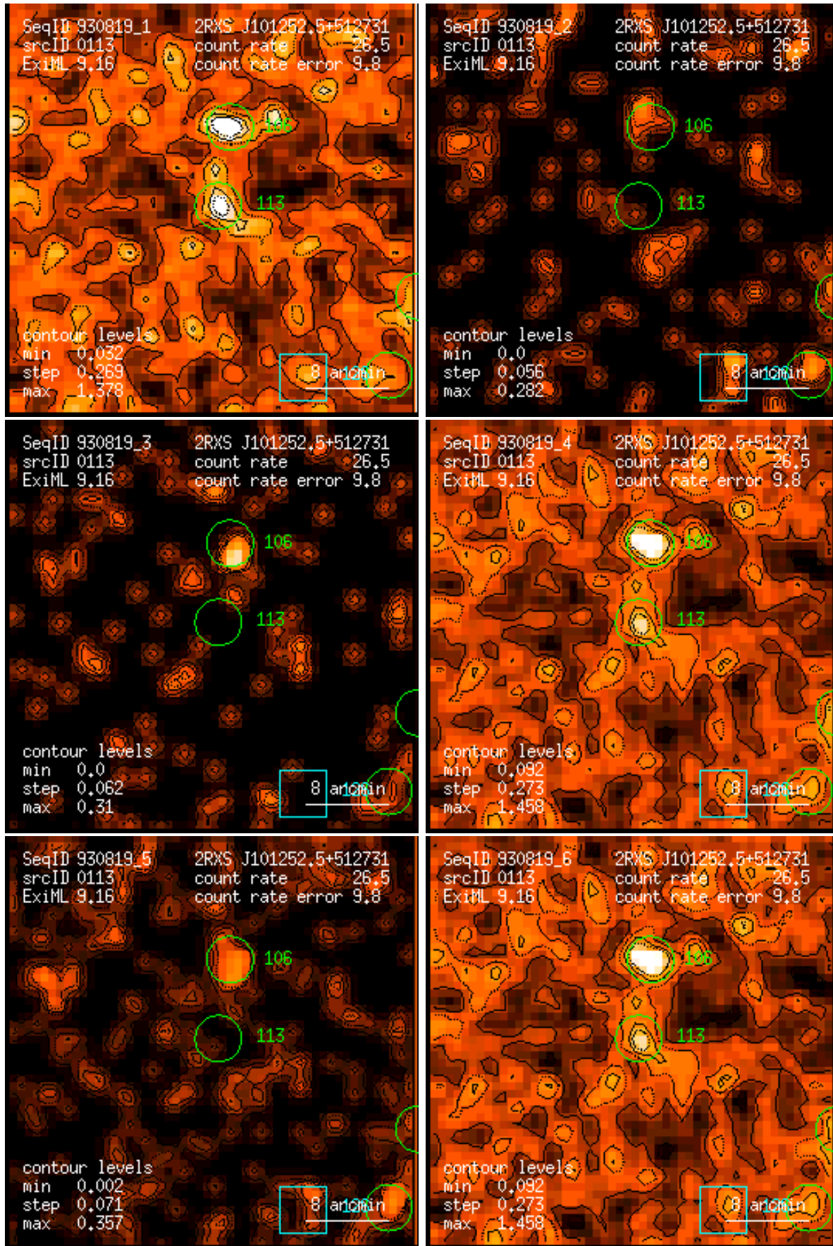
Figure 113: RASS 930819: detection 0113: band rate images, Gaussian filter: (1) PSPC channels 11 – 41, (2) 52 – 90, (3) 91 – 201, (4) 11 – 235, (5) 52 – 201, (6) 11 – 201. Broad band rates in counts/ks. Band rate contour levels in counts/ks/arcmin 2 .
