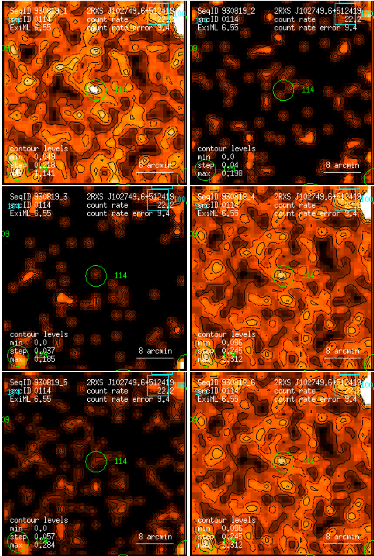
Figure 114: RASS 930819: detection 0114: band rate images, Gaussian filter: (1) PSPC channels 11 – 41, (2) 52 – 90, (3) 91 – 201, (4) 11 – 235, (5) 52 – 201, (6) 11 – 201. Broad band rates in counts/ks. Band rate contour levels in counts/ks/arcmin 2 .
