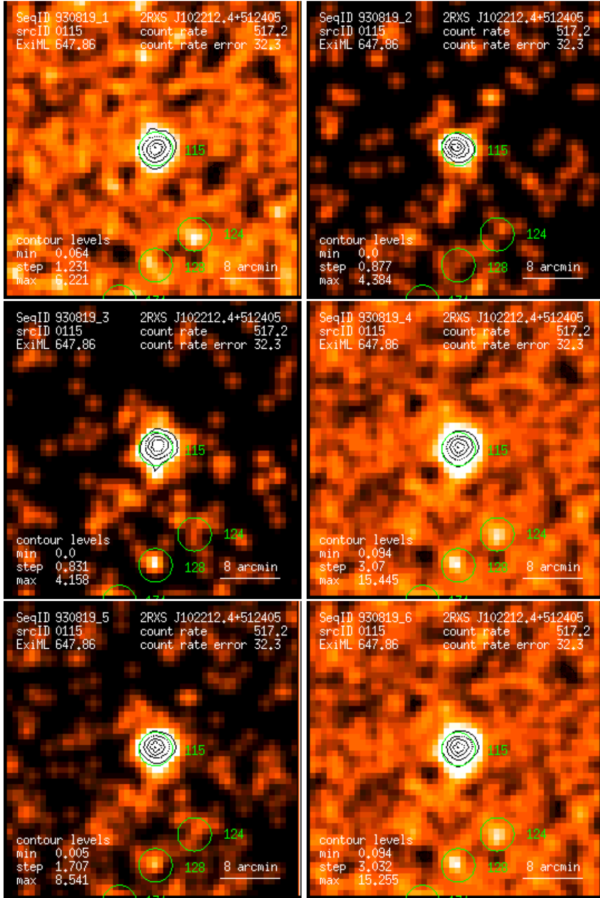
Figure 115: RASS 930819: detection 0115: band rate images, Gaussian filter: (1) PSPC channels 11 – 41, (2) 52 – 90, (3) 91 – 201, (4) 11 – 235, (5) 52 – 201, (6) 11 – 201. Broad band rates in counts/ks. Band rate contour levels in counts/ks/arcmin 2 .
