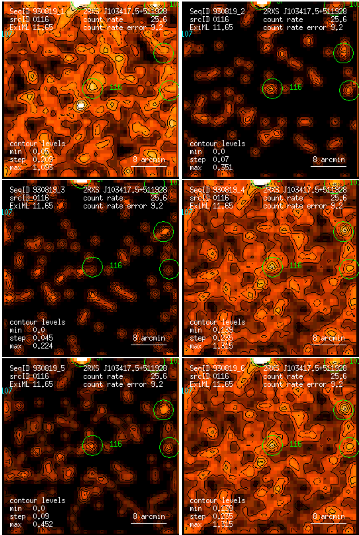
Figure 116: RASS 930819: detection 0116: band rate images, Gaussian filter: (1) PSPC channels 11 – 41, (2) 52 – 90, (3) 91 – 201, (4) 11 – 235, (5) 52 – 201, (6) 11 – 201. Broad band rates in counts/ks. Band rate contour levels in counts/ks/arcmin 2 .
