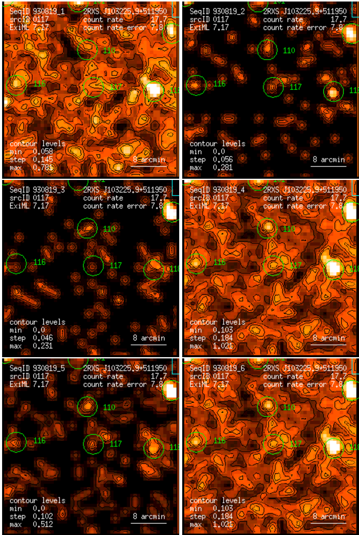
Figure 117: RASS 930819: detection 0117: band rate images, Gaussian filter: (1) PSPC channels 11 – 41, (2) 52 – 90, (3) 91 – 201, (4) 11 – 235, (5) 52 – 201, (6) 11 – 201. Broad band rates in counts/ks. Band rate contour levels in counts/ks/arcmin 2 .
