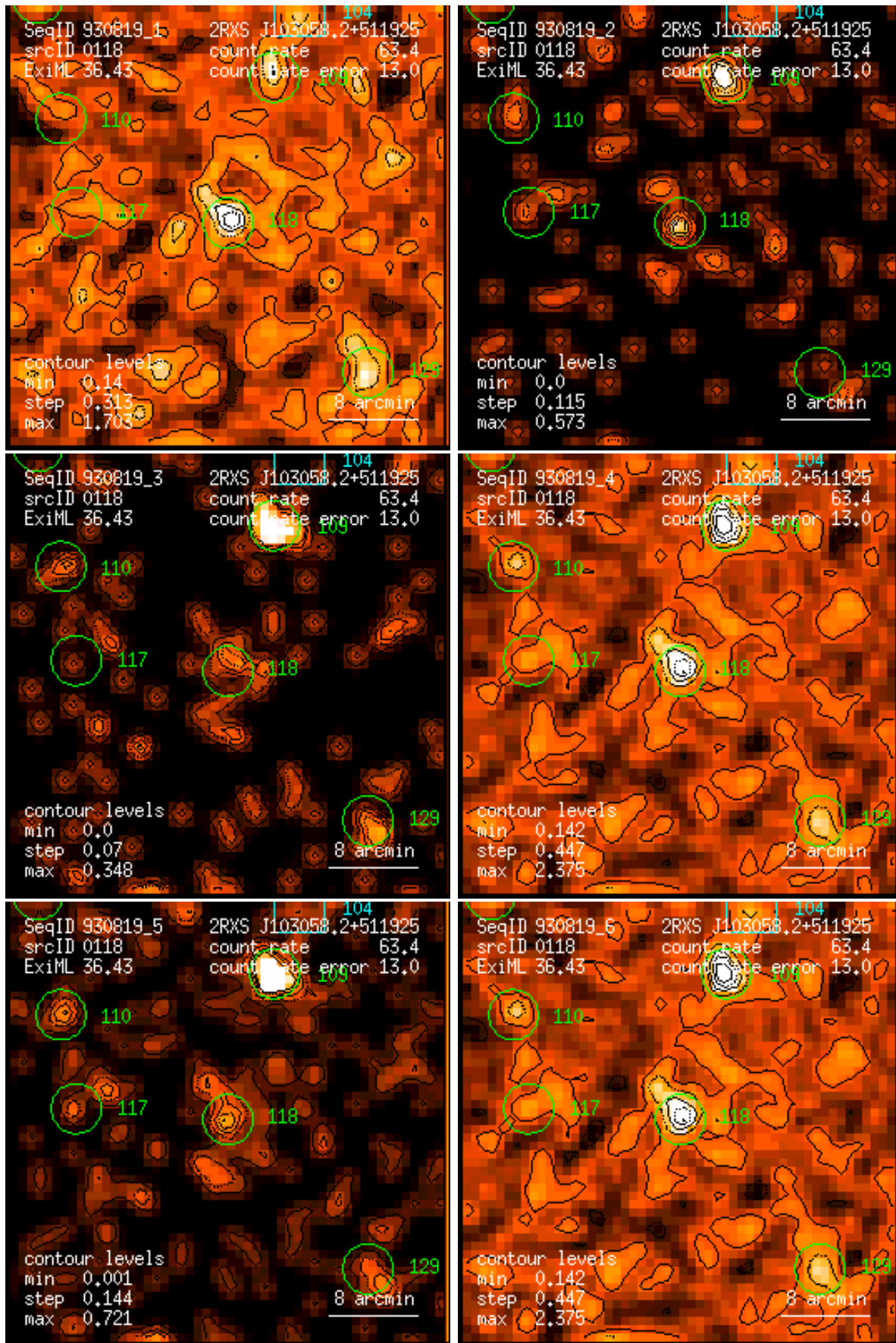
Figure 118: RASS 930819: detection 0118: band rate images, Gaussian filter: (1) PSPC channels 11 – 41, (2) 52 – 90, (3) 91 – 201, (4) 11 – 235, (5) 52 – 201, (6) 11 – 201. Broad band rates in counts/ks. Band rate contour levels in counts/ks/arcmin 2 .
