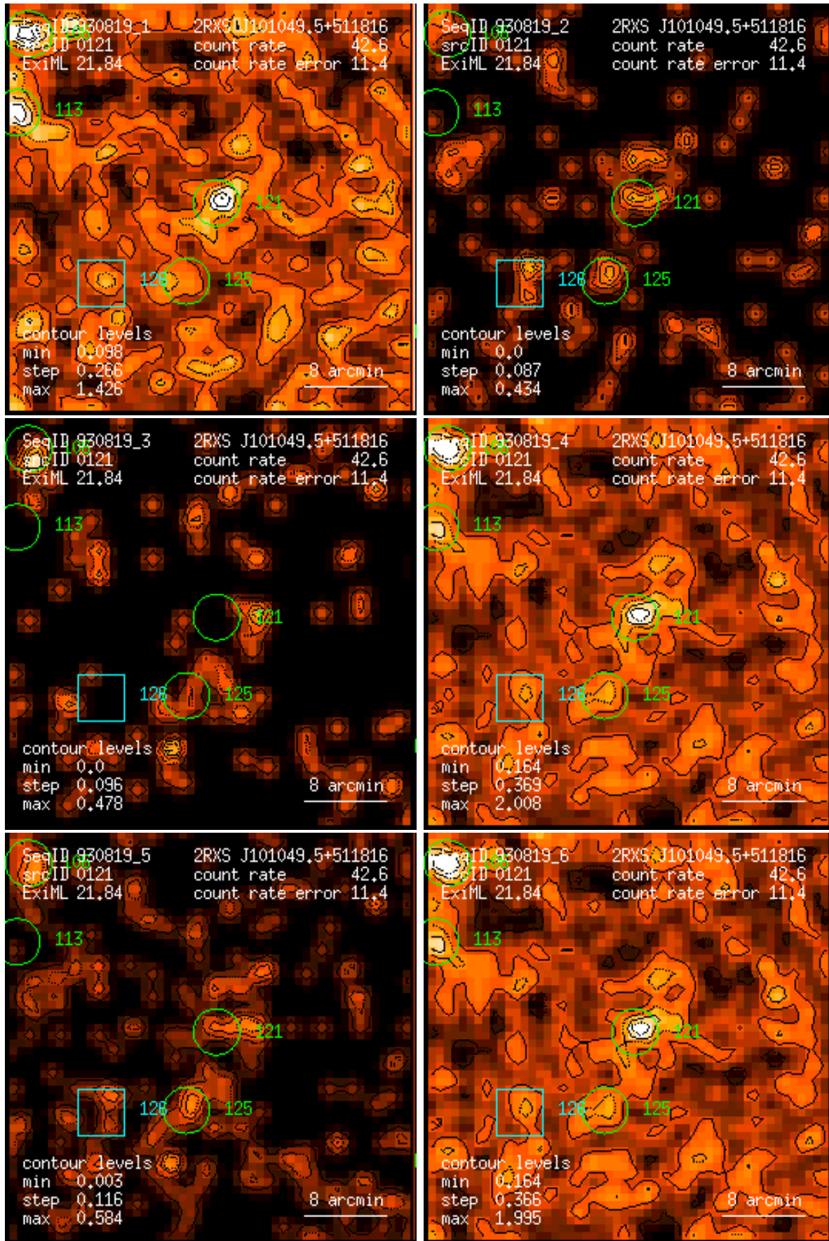
Figure 121: RASS 930819: detection 0121: band rate images, Gaussian filter: (1) PSPC channels 11 – 41, (2) 52 – 90, (3) 91 – 201, (4) 11 – 235, (5) 52 – 201, (6) 11 – 201. Broad band rates in counts/ks. Band rate contour levels in counts/ks/arcmin 2 .
