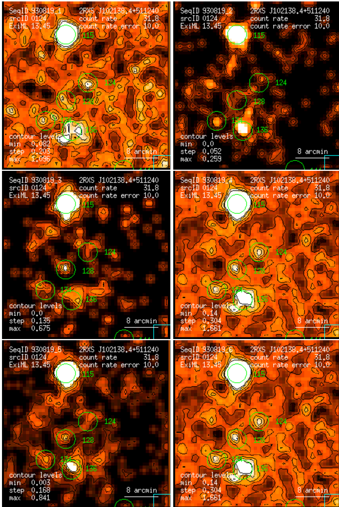
Figure 124: RASS 930819: detection 0124: band rate images, Gaussian filter: (1) PSPC channels 11 – 41, (2) 52 – 90, (3) 91 – 201, (4) 11 – 235, (5) 52 – 201, (6) 11 – 201. Broad band rates in counts/ks. Band rate contour levels in counts/ks/arcmin 2 .
