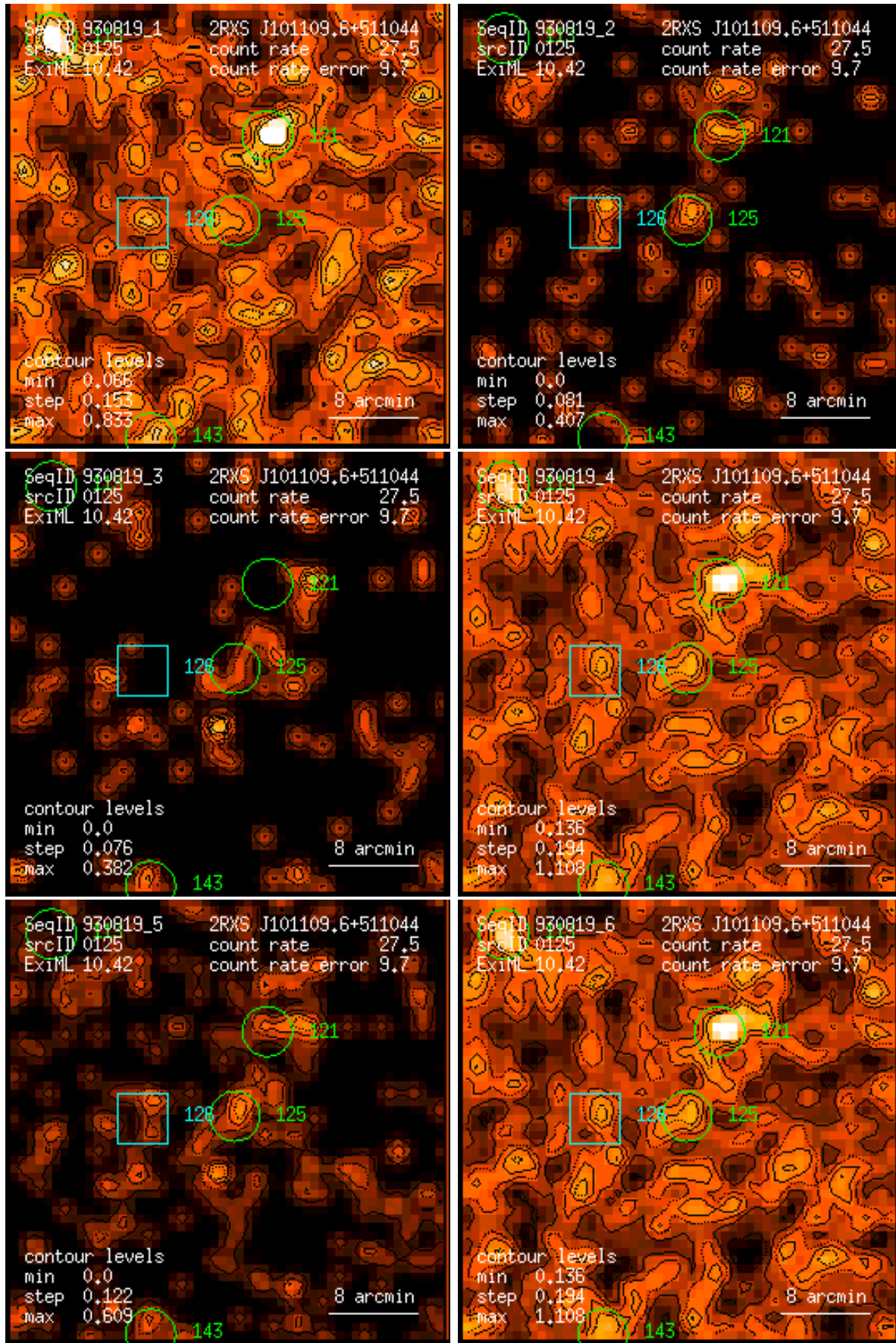
Figure 125: RASS 930819: detection 0125: band rate images, Gaussian filter: (1) PSPC channels 11 – 41, (2) 52 – 90, (3) 91 – 201, (4) 11 – 235, (5) 52 – 201, (6) 11 – 201. Broad band rates in counts/ks. Band rate contour levels in counts/ks/arcmin 2 .
