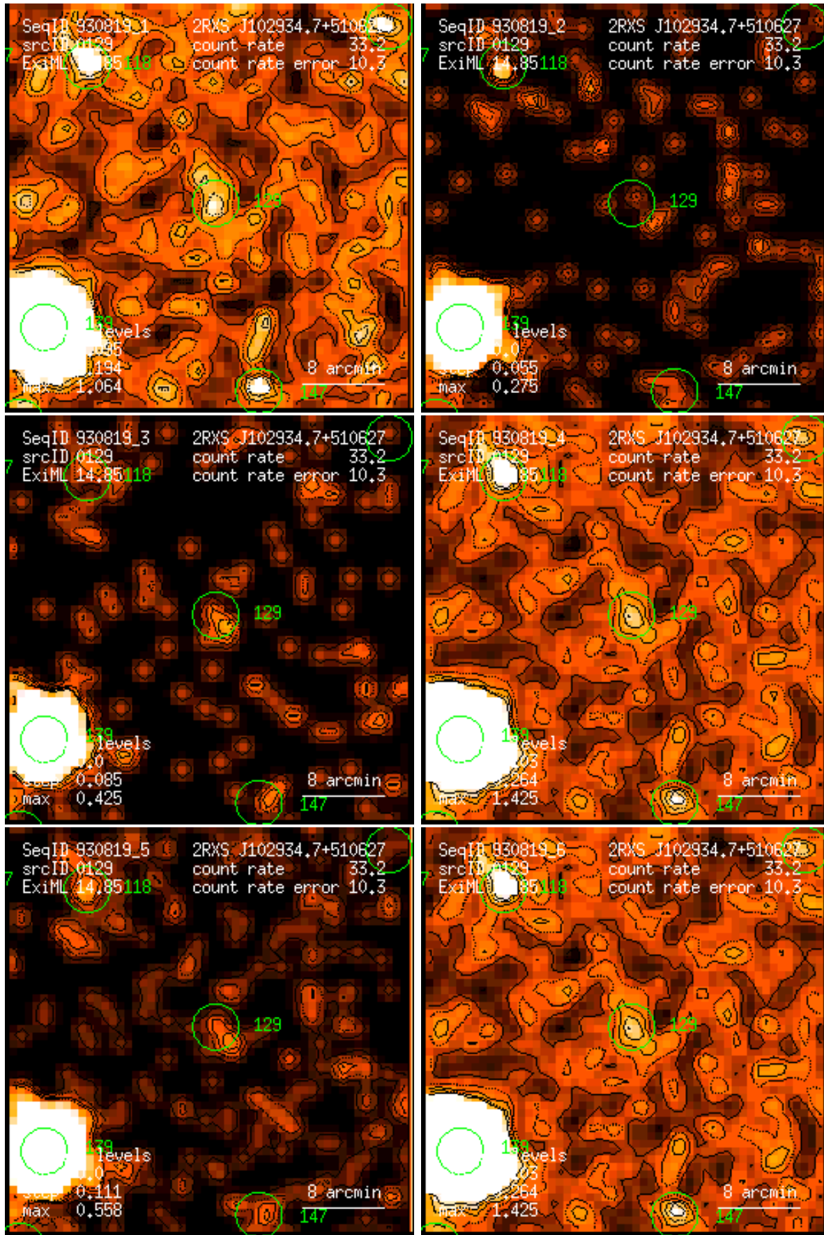
Figure 129: RASS 930819: detection 0129: band rate images, Gaussian filter: (1) PSPC channels 11 – 41, (2) 52 – 90, (3) 91 – 201, (4) 11 – 235, (5) 52 – 201, (6) 11 – 201. Broad band rates in counts/ks. Band rate contour levels in counts/ks/arcmin 2 .
