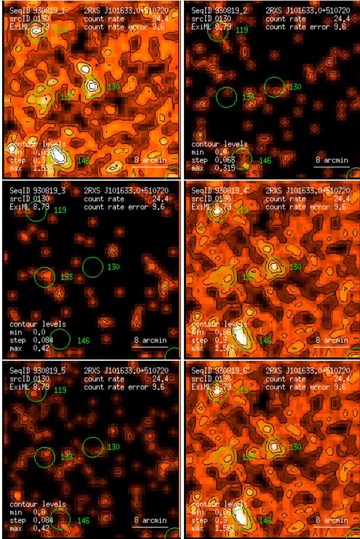
Figure 130: RASS 930819: detection 0130: band rate images, Gaussian filter: (1) PSPC channels 11 – 41, (2) 52 – 90, (3) 91 – 201, (4) 11 – 235, (5) 52 – 201, (6) 11 – 201. Broad band rates in counts/ks. Band rate contour levels in counts/ks/arcmin 2 .
