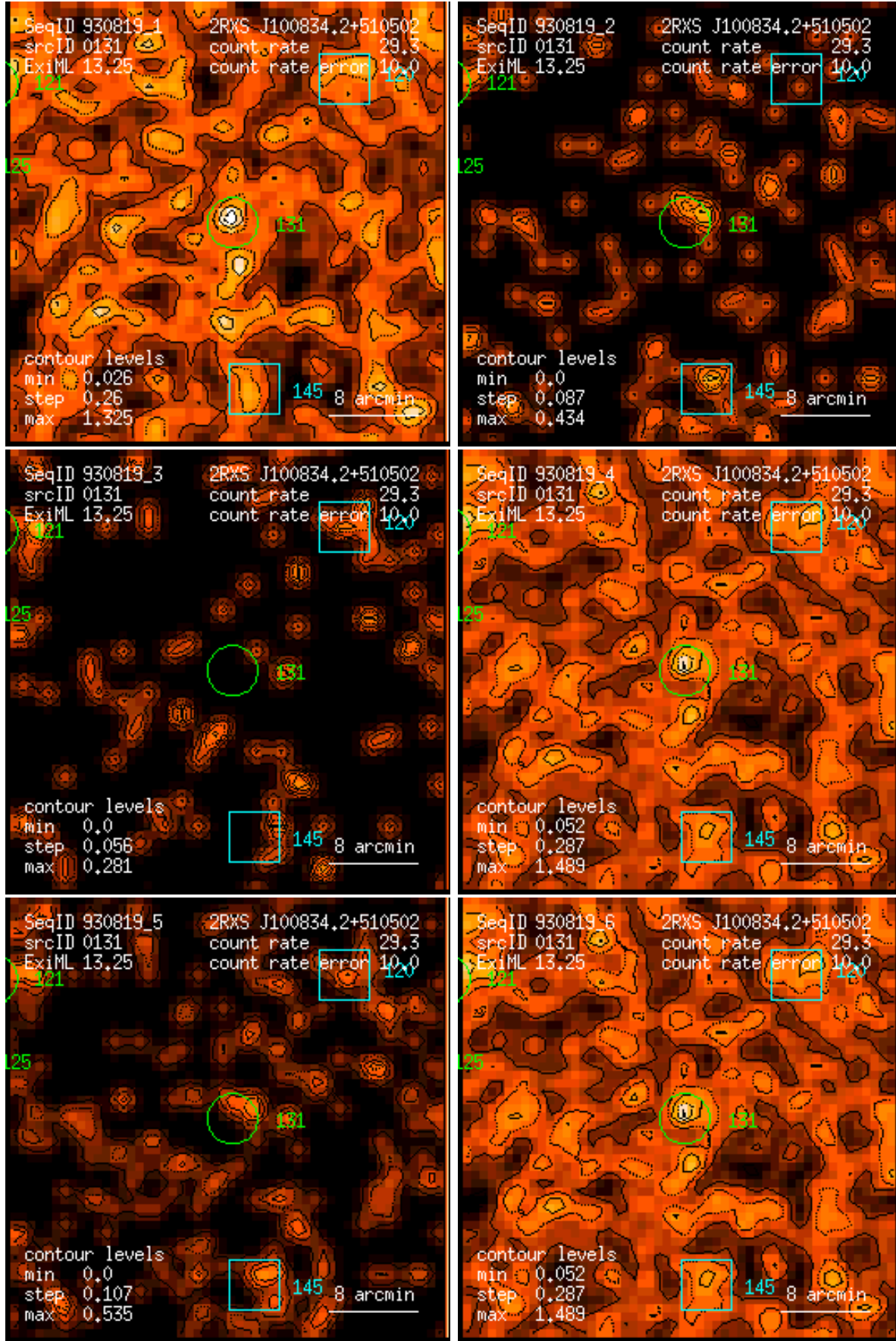
Figure 131: RASS 930819: detection 0131: band rate images, Gaussian filter: (1) PSPC channels 11 – 41, (2) 52 – 90, (3) 91 – 201, (4) 11 – 235, (5) 52 – 201, (6) 11 – 201. Broad band rates in counts/ks. Band rate contour levels in counts/ks/arcmin 2 .
