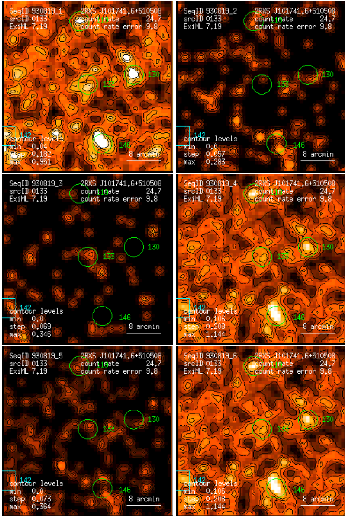
Figure 133: RASS 930819: detection 0133: band rate images, Gaussian filter: (1) PSPC channels 11 – 41, (2) 52 – 90, (3) 91 – 201, (4) 11 – 235, (5) 52 – 201, (6) 11 – 201. Broad band rates in counts/ks. Band rate contour levels in counts/ks/arcmin 2 .
