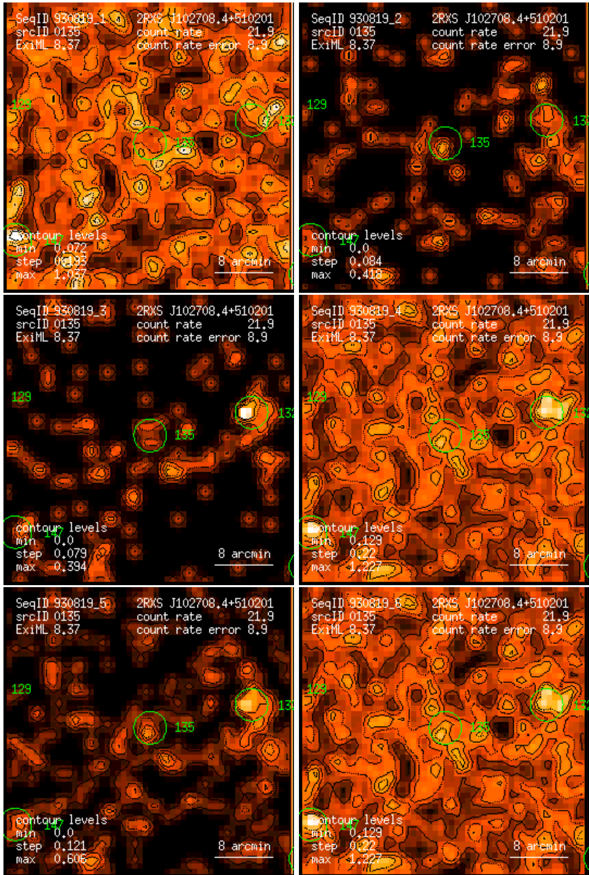
Figure 135: RASS 930819: detection 0135: band rate images, Gaussian filter: (1) PSPC channels 11 – 41, (2) 52 – 90, (3) 91 – 201, (4) 11 – 235, (5) 52 – 201, (6) 11 – 201. Broad band rates in counts/ks. Band rate contour levels in counts/ks/arcmin 2 .
