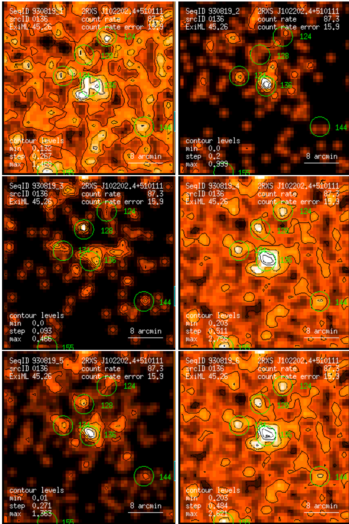
Figure 136: RASS 930819: detection 0136: band rate images, Gaussian filter: (1) PSPC channels 11 – 41, (2) 52 – 90, (3) 91 – 201, (4) 11 – 235, (5) 52 – 201, (6) 11 – 201. Broad band rates in counts/ks. Band rate contour levels in counts/ks/arcmin 2 .
