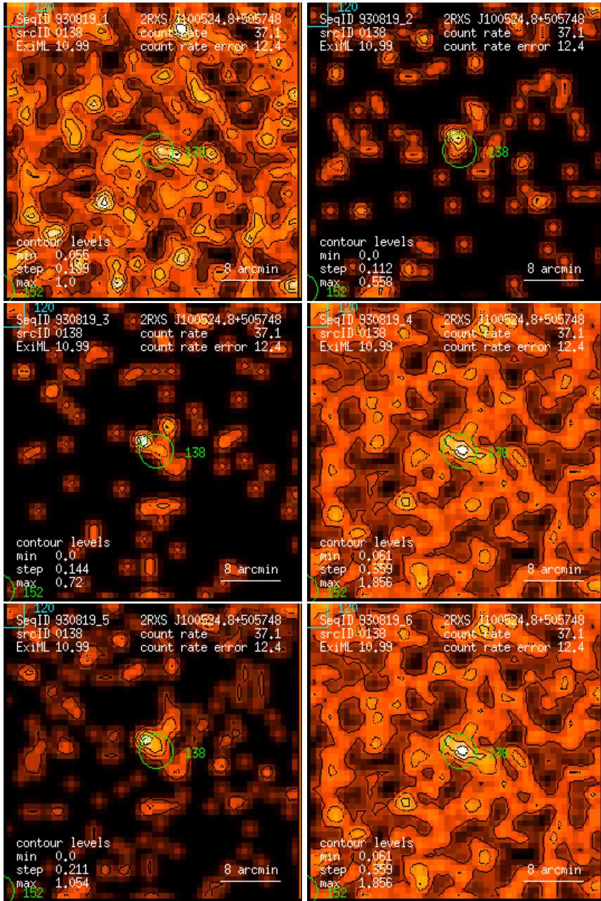
Figure 138: RASS 930819: detection 0138: band rate images, Gaussian filter: (1) PSPC channels 11 – 41, (2) 52 – 90, (3) 91 – 201, (4) 11 – 235, (5) 52 – 201, (6) 11 – 201. Broad band rates in counts/ks. Band rate contour levels in counts/ks/arcmin 2 .
