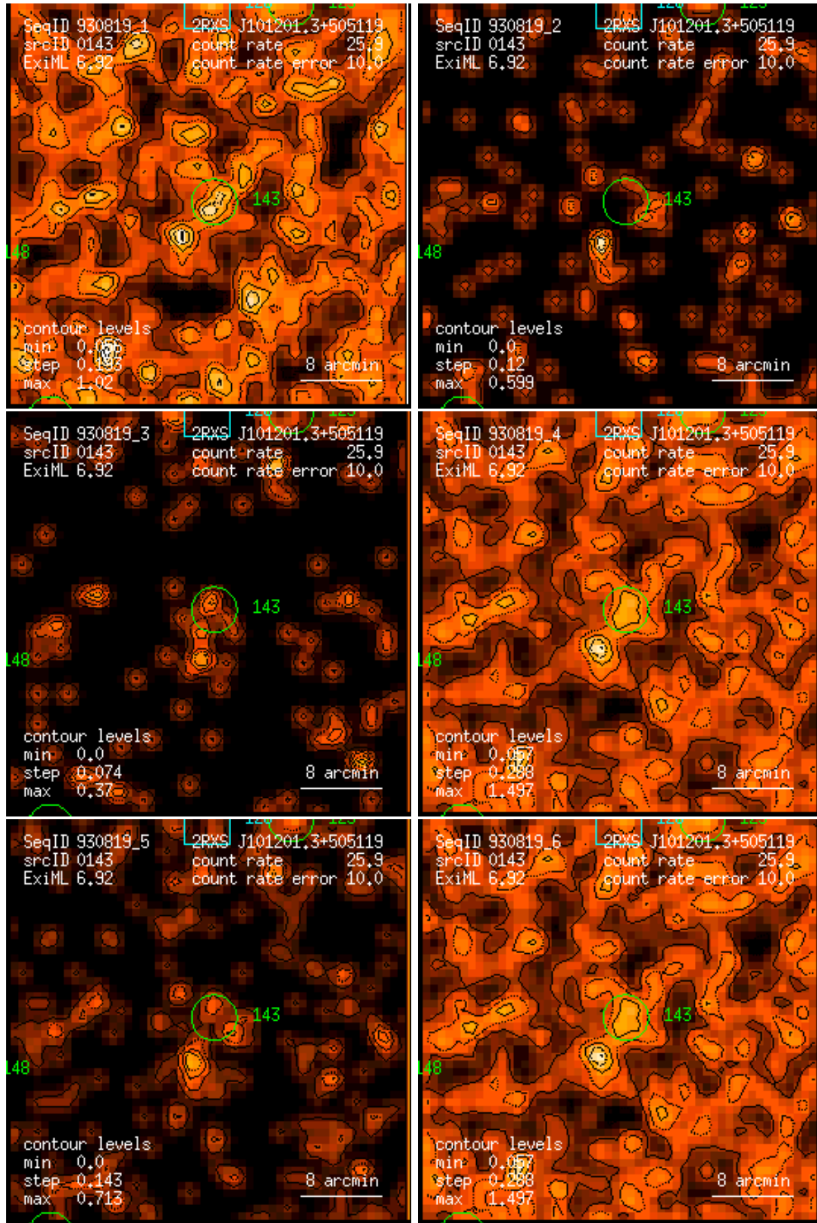
Figure 143: RASS 930819: detection 0143: band rate images, Gaussian filter: (1) PSPC channels 11 – 41, (2) 52 – 90, (3) 91 – 201, (4) 11 – 235, (5) 52 – 201, (6) 11 – 201. Broad band rates in counts/ks. Band rate contour levels in counts/ks/arcmin 2 .
