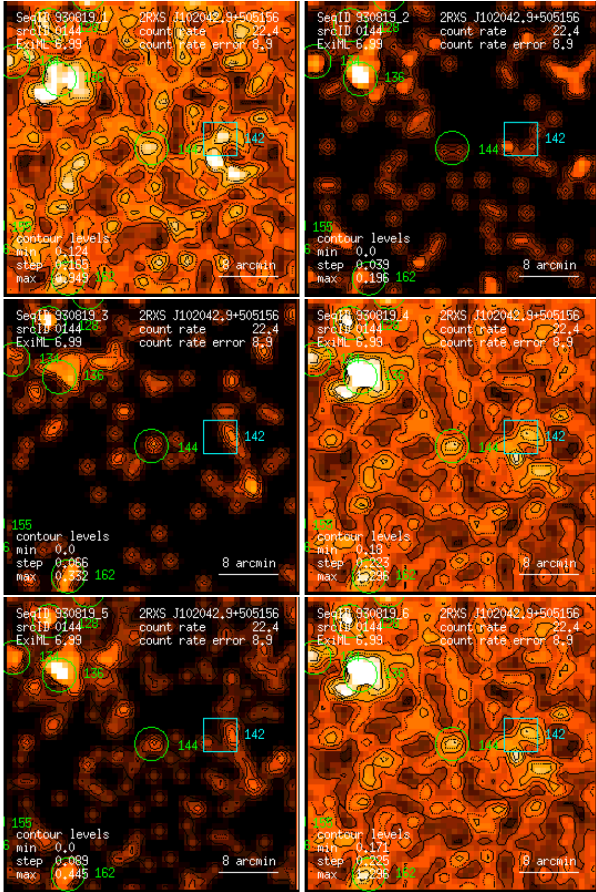
Figure 144: RASS 930819: detection 0144: band rate images, Gaussian filter: (1) PSPC channels 11 – 41, (2) 52 – 90, (3) 91 – 201, (4) 11 – 235, (5) 52 – 201, (6) 11 – 201. Broad band rates in counts/ks. Band rate contour levels in counts/ks/arcmin 2 .
