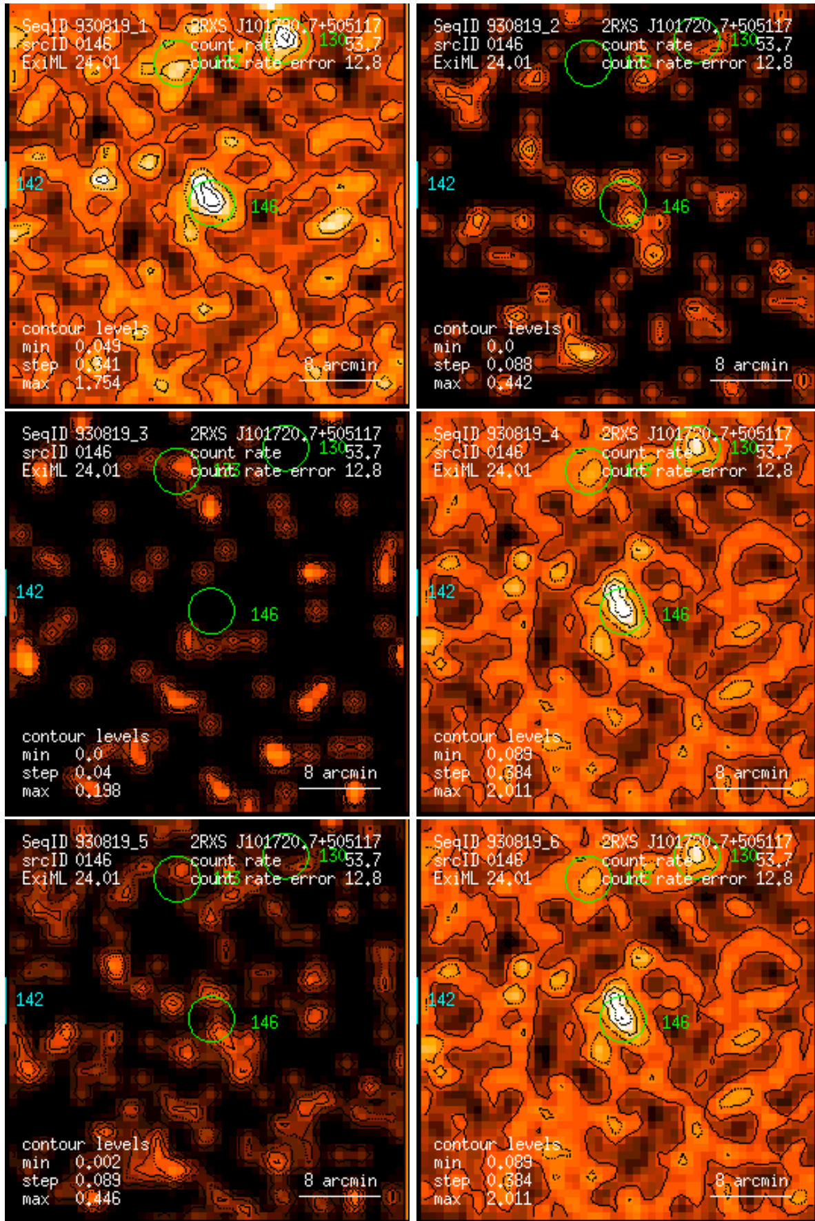
Figure 146: RASS 930819: detection 0146: band rate images, Gaussian filter: (1) PSPC channels 11 – 41, (2) 52 – 90, (3) 91 – 201, (4) 11 – 235, (5) 52 – 201, (6) 11 – 201. Broad band rates in counts/ks. Band rate contour levels in counts/ks/arcmin 2 .
