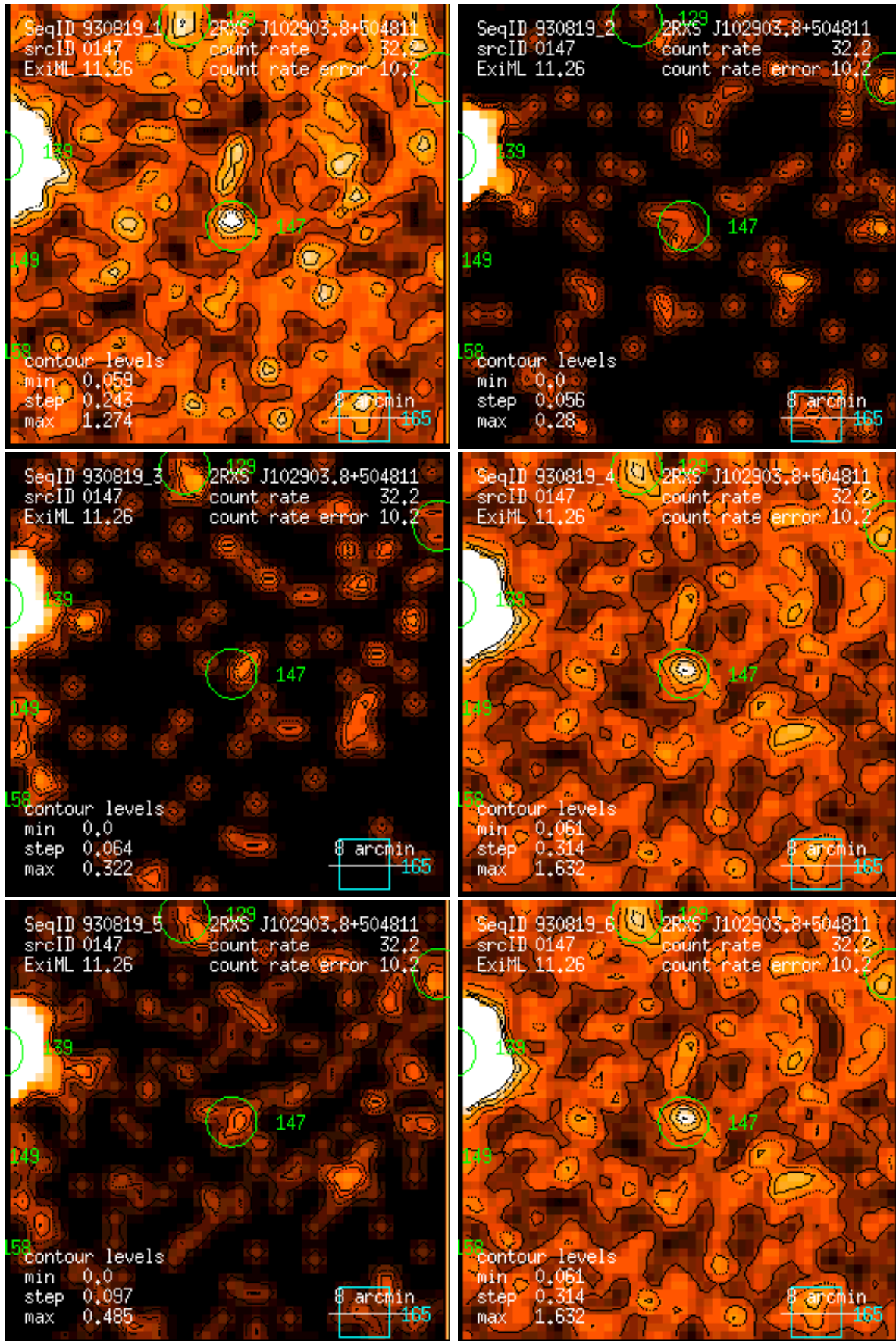
Figure 147: RASS 930819: detection 0147: band rate images, Gaussian filter: (1) PSPC channels 11 – 41, (2) 52 – 90, (3) 91 – 201, (4) 11 – 235, (5) 52 – 201, (6) 11 – 201. Broad band rates in counts/ks. Band rate contour levels in counts/ks/arcmin 2 .
