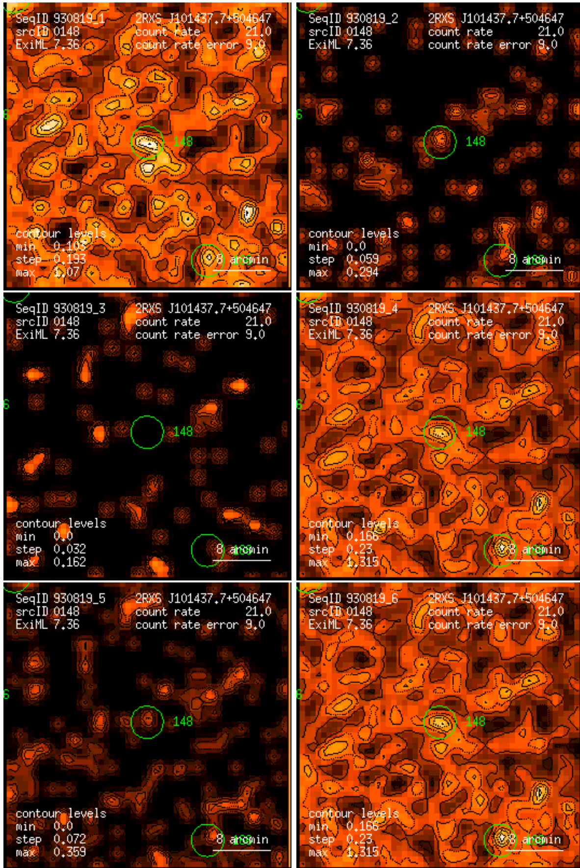
Figure 148: RASS 930819: detection 0148: band rate images, Gaussian filter: (1) PSPC channels 11 – 41, (2) 52 – 90, (3) 91 – 201, (4) 11 – 235, (5) 52 – 201, (6) 11 – 201. Broad band rates in counts/ks. Band rate contour levels in counts/ks/arcmin 2 .
