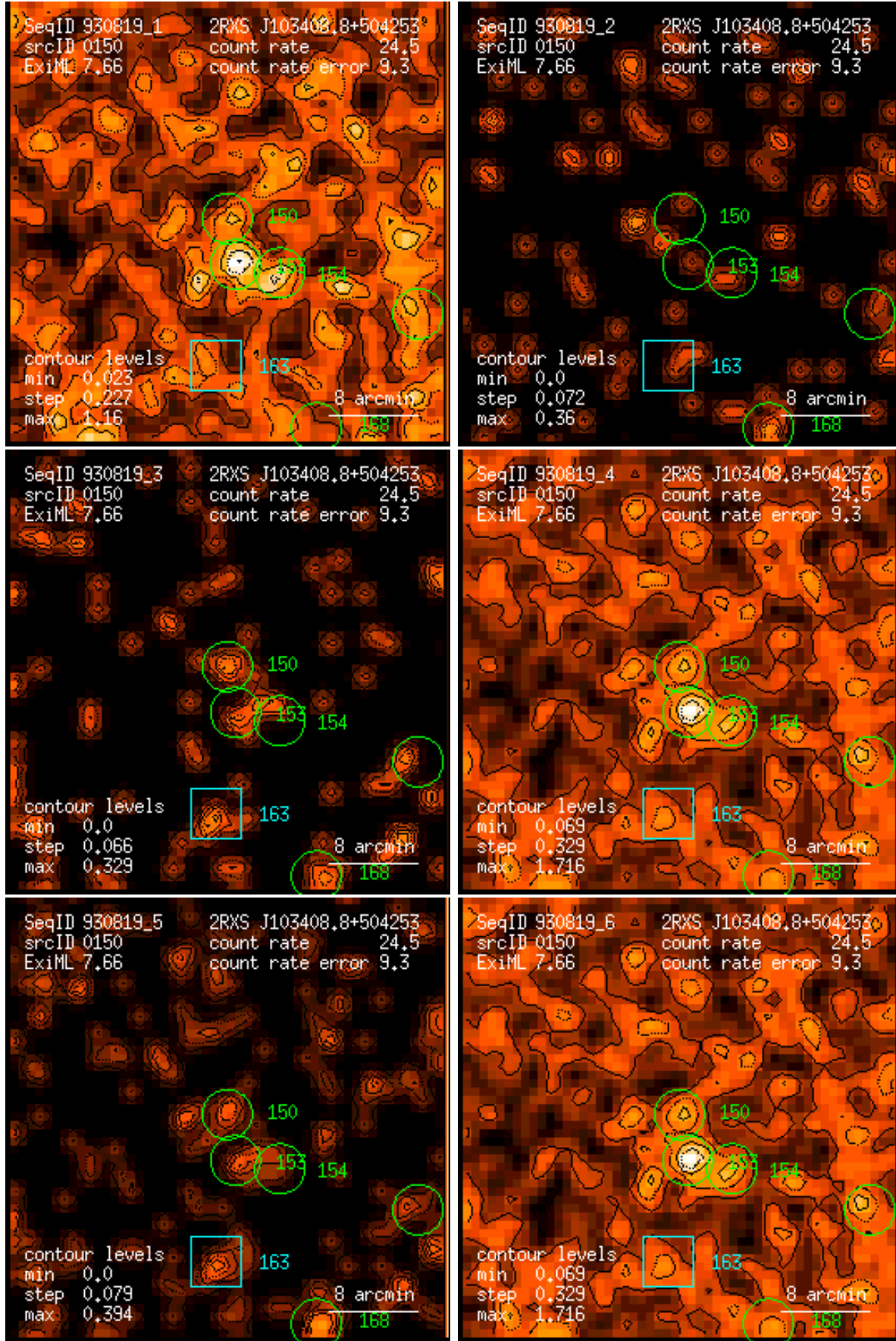
Figure 150: RASS 930819: detection 0150: band rate images, Gaussian filter: (1) PSPC channels 11 – 41, (2) 52 – 90, (3) 91 – 201, (4) 11 – 235, (5) 52 – 201, (6) 11 – 201. Broad band rates in counts/ks. Band rate contour levels in counts/ks/arcmin 2 .
