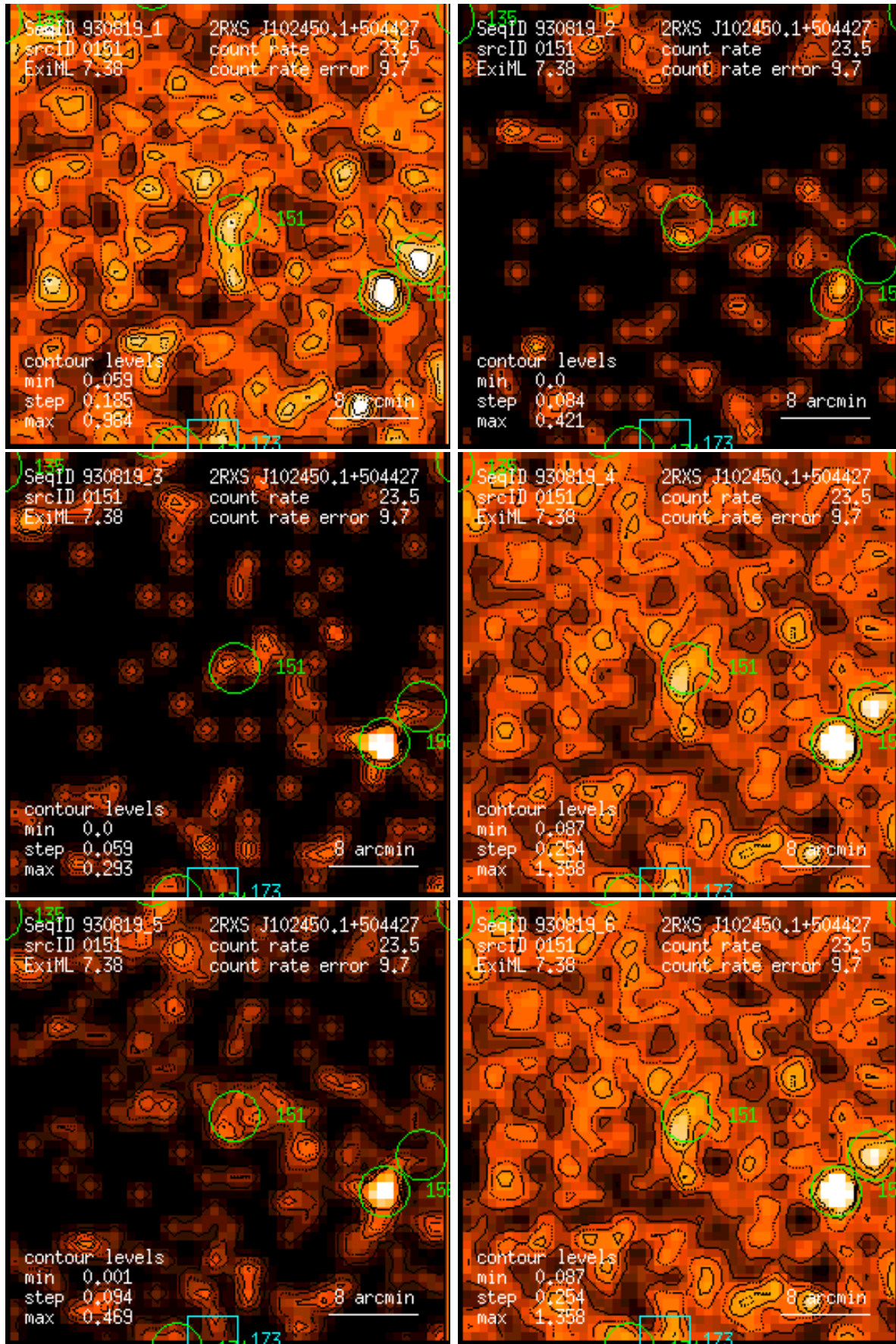
Figure 151: RASS 930819: detection 0151: band rate images, Gaussian filter: (1) PSPC channels 11 – 41, (2) 52 – 90, (3) 91 – 201, (4) 11 – 235, (5) 52 – 201, (6) 11 – 201. Broad band rates in counts/ks. Band rate contour levels in counts/ks/arcmin 2 .
