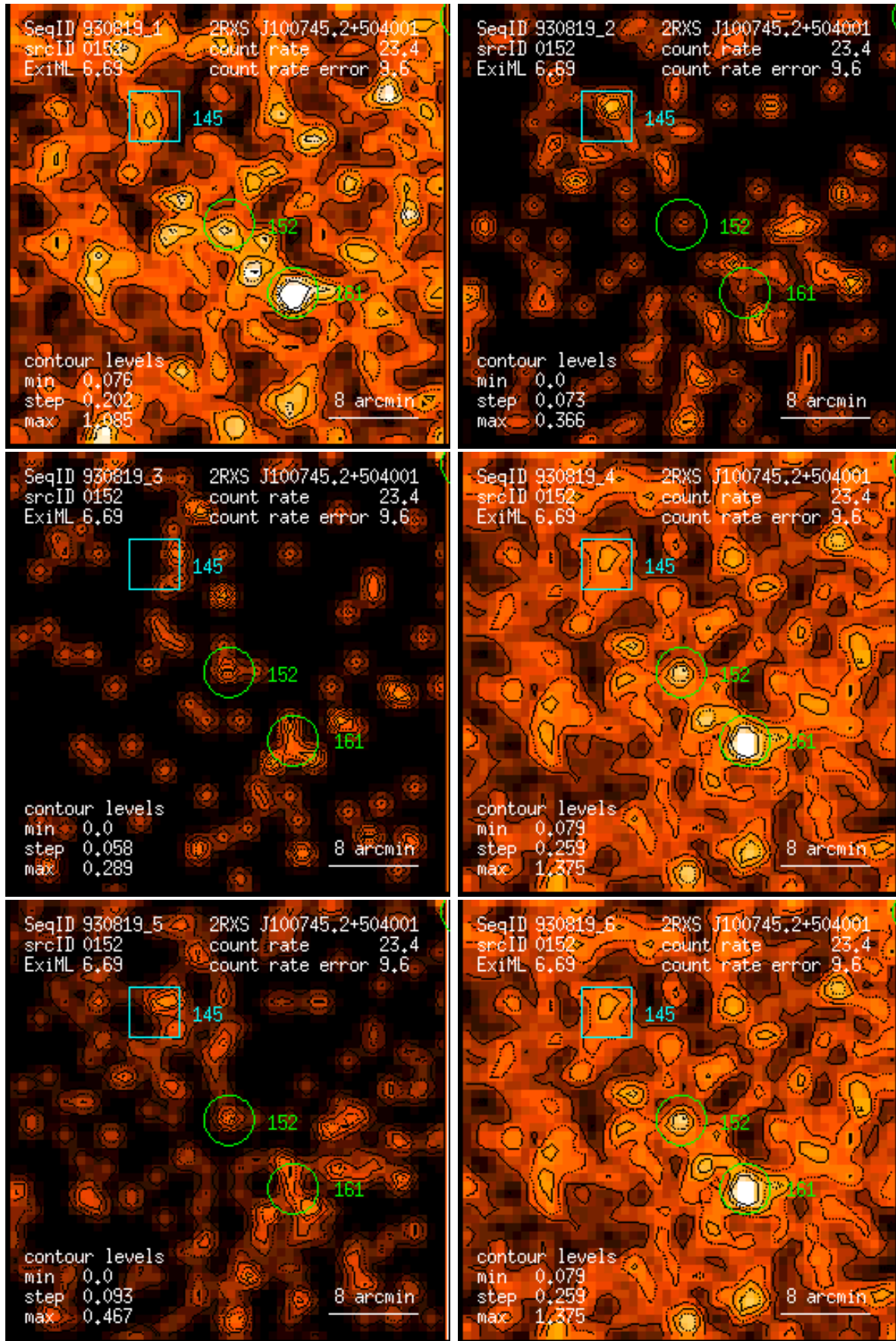
Figure 152: RASS 930819: detection 0152: band rate images, Gaussian filter: (1) PSPC channels 11 – 41, (2) 52 – 90, (3) 91 – 201, (4) 11 – 235, (5) 52 – 201, (6) 11 – 201. Broad band rates in counts/ks. Band rate contour levels in counts/ks/arcmin 2 .
