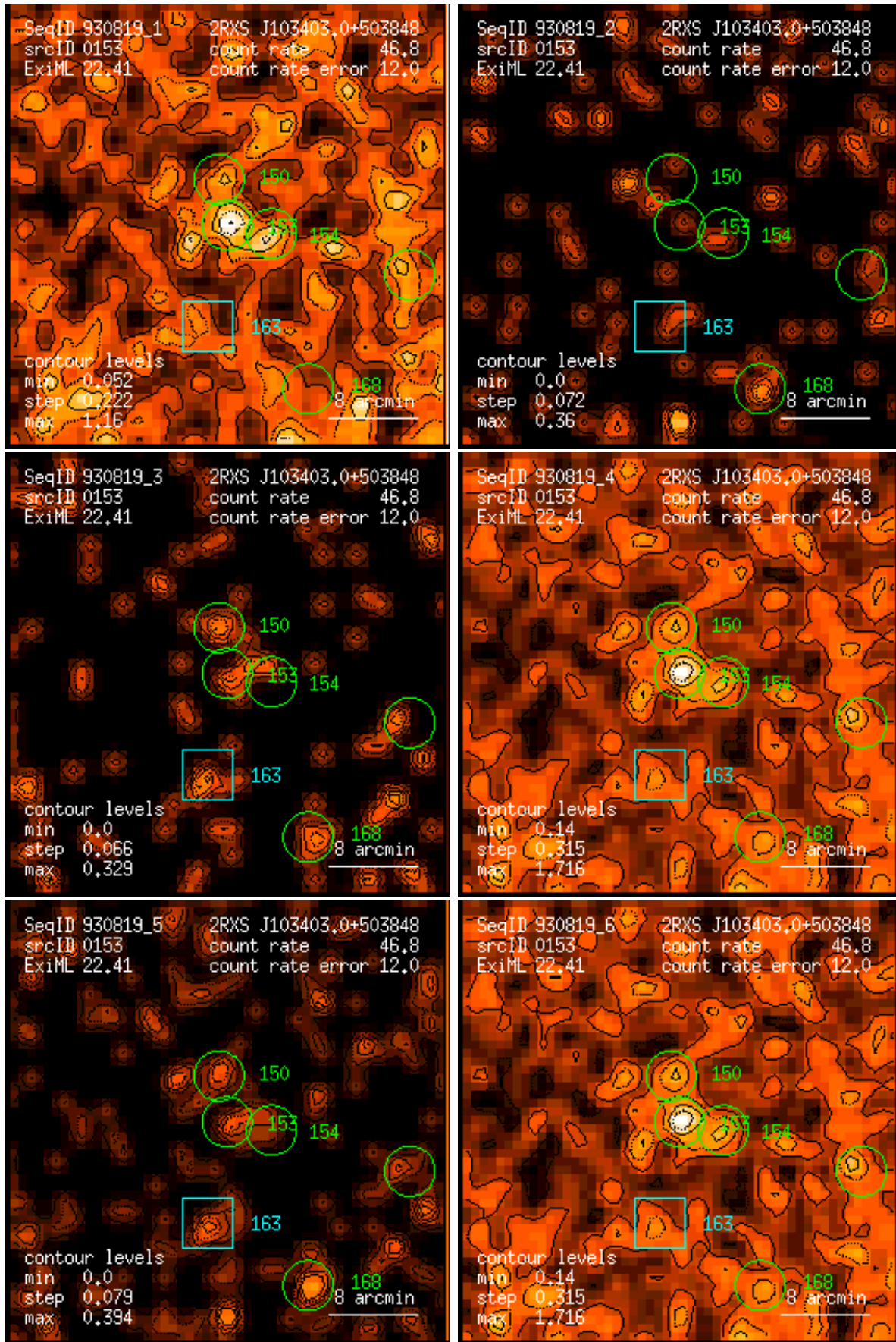
Figure 153: RASS 930819: detection 0153: band rate images, Gaussian filter: (1) PSPC channels 11 – 41, (2) 52 – 90, (3) 91 – 201, (4) 11 – 235, (5) 52 – 201, (6) 11 – 201. Broad band rates in counts/ks. Band rate contour levels in counts/ks/arcmin 2 .
