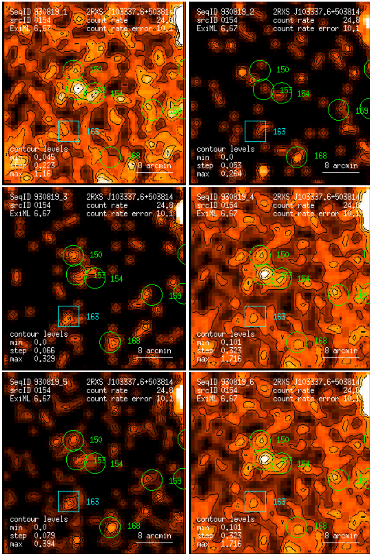
Figure 154: RASS 930819: detection 0154: band rate images, Gaussian filter: (1) PSPC channels 11 – 41, (2) 52 – 90, (3) 91 – 201, (4) 11 – 235, (5) 52 – 201, (6) 11 – 201. Broad band rates in counts/ks. Band rate contour levels in counts/ks/arcmin 2 .
