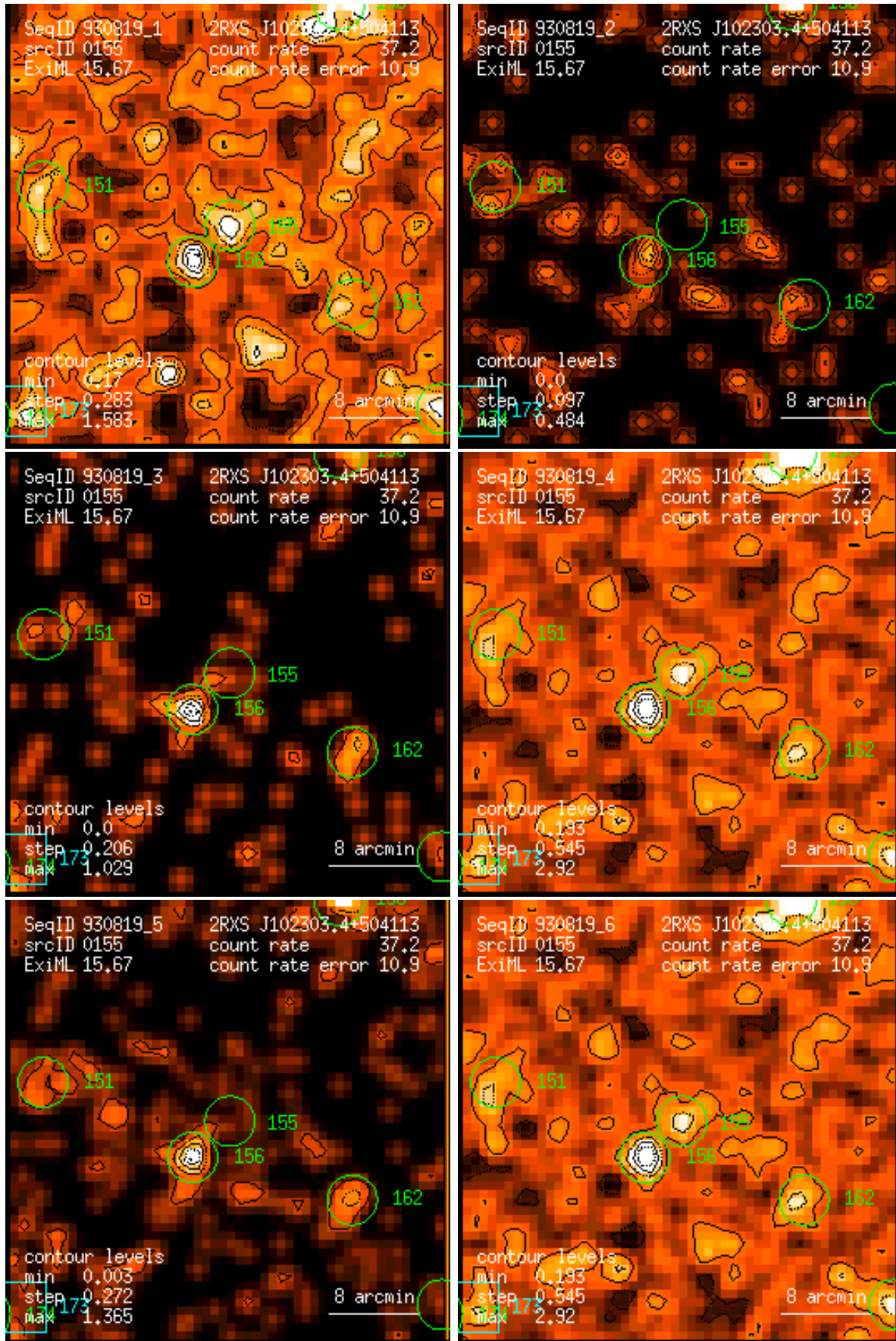
Figure 155: RASS 930819: detection 0155: band rate images, Gaussian filter: (1) PSPC channels 11 – 41, (2) 52 – 90, (3) 91 – 201, (4) 11 – 235, (5) 52 – 201, (6) 11 – 201. Broad band rates in counts/ks. Band rate contour levels in counts/ks/arcmin 2 .
