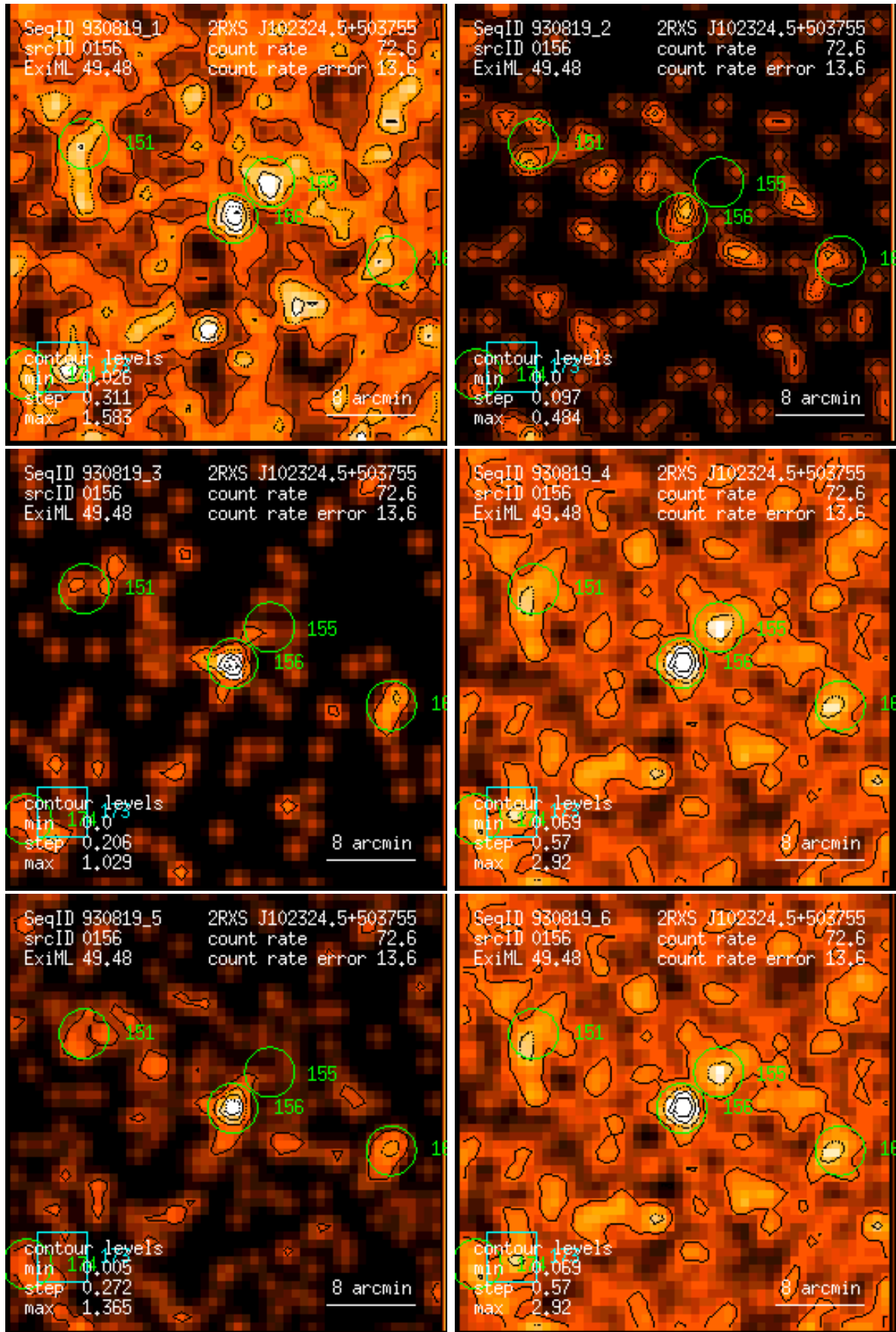
Figure 156: RASS 930819: detection 0156: band rate images, Gaussian filter: (1) PSPC channels 11 – 41, (2) 52 – 90, (3) 91 – 201, (4) 11 – 235, (5) 52 – 201, (6) 11 – 201. Broad band rates in counts/ks. Band rate contour levels in counts/ks/arcmin 2 .
