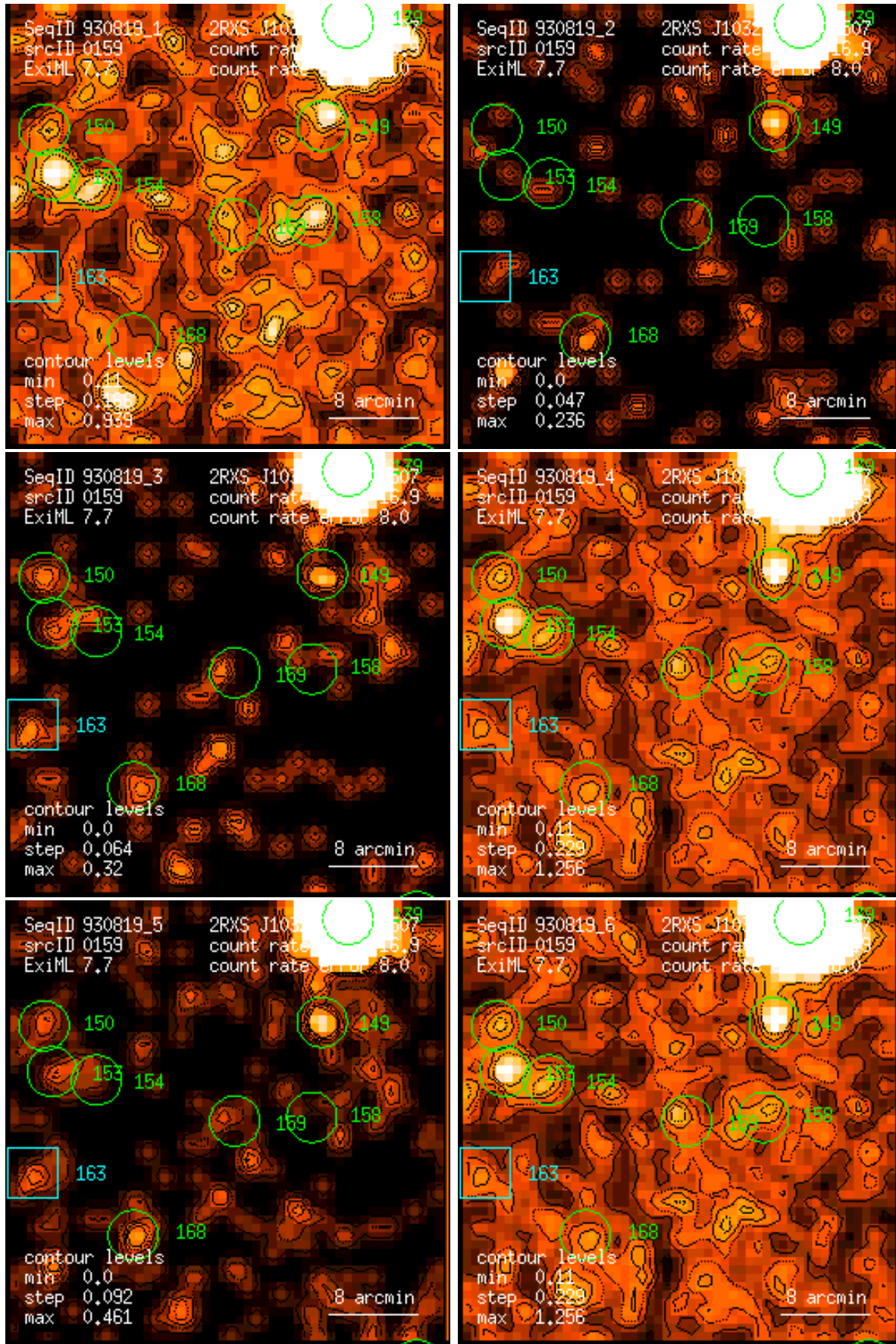
Figure 159: RASS 930819: detection 0159: band rate images, Gaussian filter: (1) PSPC channels 11 – 41, (2) 52 – 90, (3) 91 – 201, (4) 11 – 235, (5) 52 – 201, (6) 11 – 201. Broad band rates in counts/ks. Band rate contour levels in counts/ks/arcmin 2 .
