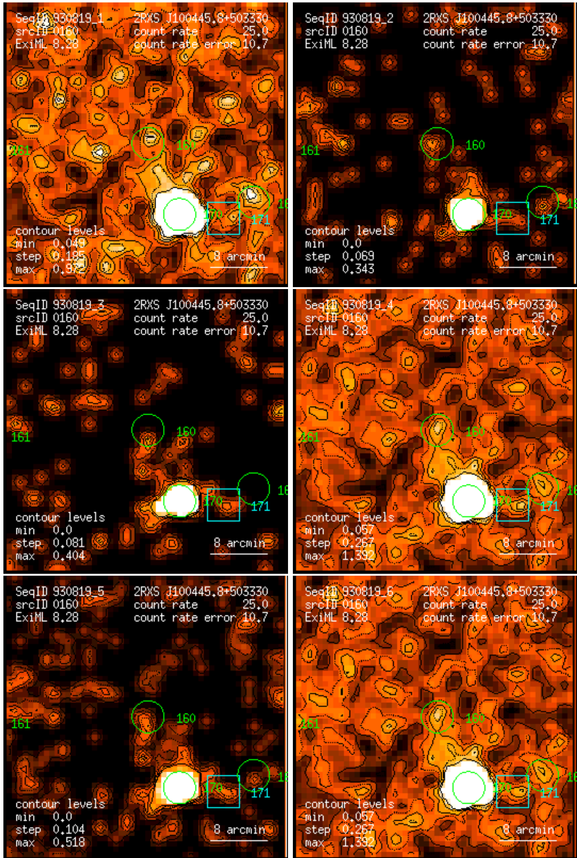
Figure 160: RASS 930819: detection 0160: band rate images, Gaussian filter: (1) PSPC channels 11 – 41, (2) 52 – 90, (3) 91 – 201, (4) 11 – 235, (5) 52 – 201, (6) 11 – 201. Broad band rates in counts/ks. Band rate contour levels in counts/ks/arcmin 2 .
