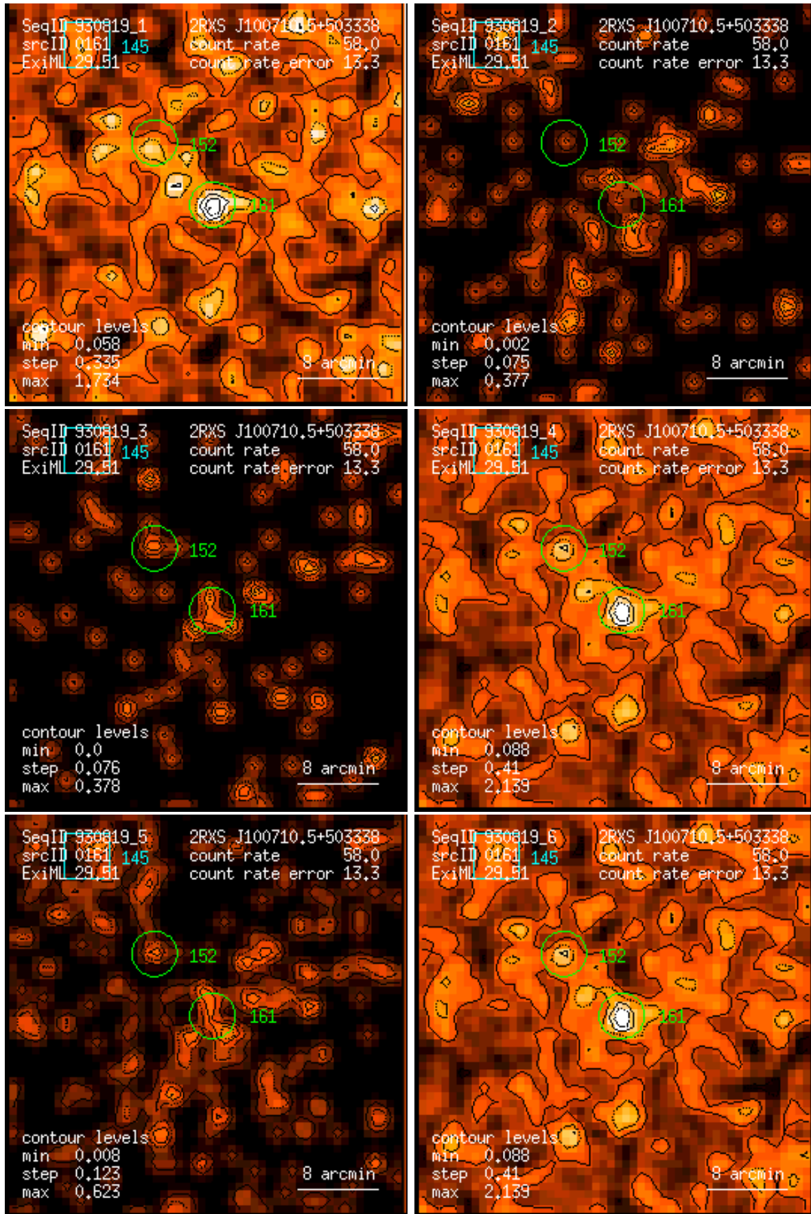
Figure 161: RASS 930819: detection 0161: band rate images, Gaussian filter: (1) PSPC channels 11 – 41, (2) 52 – 90, (3) 91 – 201, (4) 11 – 235, (5) 52 – 201, (6) 11 – 201. Broad band rates in counts/ks. Band rate contour levels in counts/ks/arcmin 2 .
