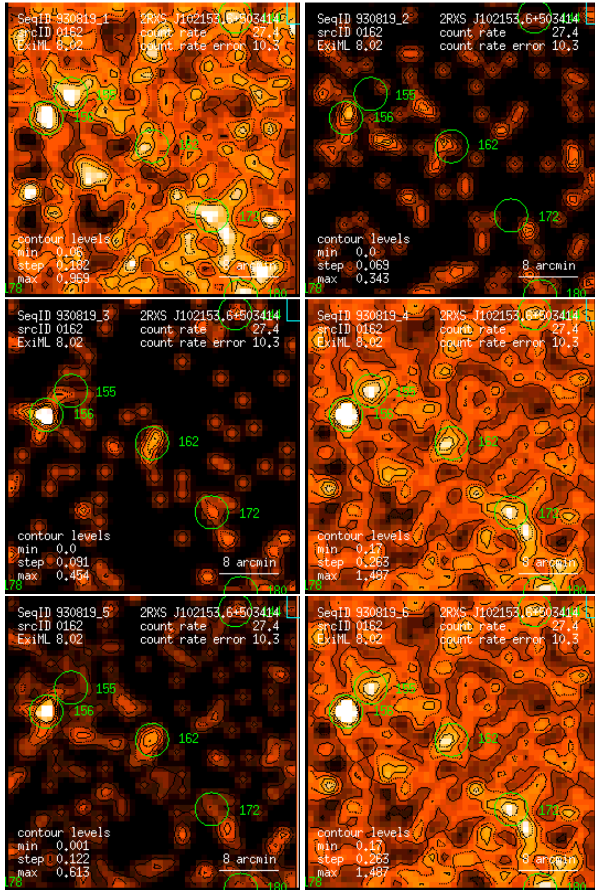
Figure 162: RASS 930819: detection 0162: band rate images, Gaussian filter: (1) PSPC channels 11 – 41, (2) 52 – 90, (3) 91 – 201, (4) 11 – 235, (5) 52 – 201, (6) 11 – 201. Broad band rates in counts/ks. Band rate contour levels in counts/ks/arcmin 2 .
