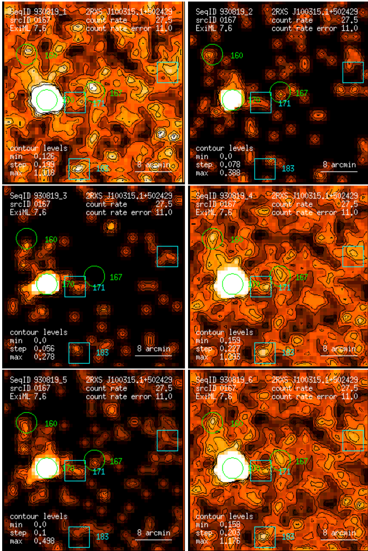
Figure 167: RASS 930819: detection 0167: band rate images, Gaussian filter: (1) PSPC channels 11 – 41, (2) 52 – 90, (3) 91 – 201, (4) 11 – 235, (5) 52 – 201, (6) 11 – 201. Broad band rates in counts/ks. Band rate contour levels in counts/ks/arcmin 2 .
