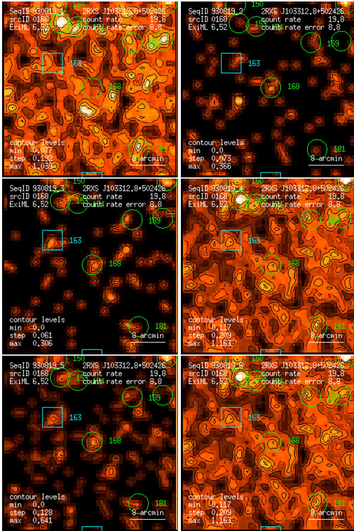
Figure 168: RASS 930819: detection 0168: band rate images, Gaussian filter: (1) PSPC channels 11 – 41, (2) 52 – 90, (3) 91 – 201, (4) 11 – 235, (5) 52 – 201, (6) 11 – 201. Broad band rates in counts/ks. Band rate contour levels in counts/ks/arcmin 2 .
