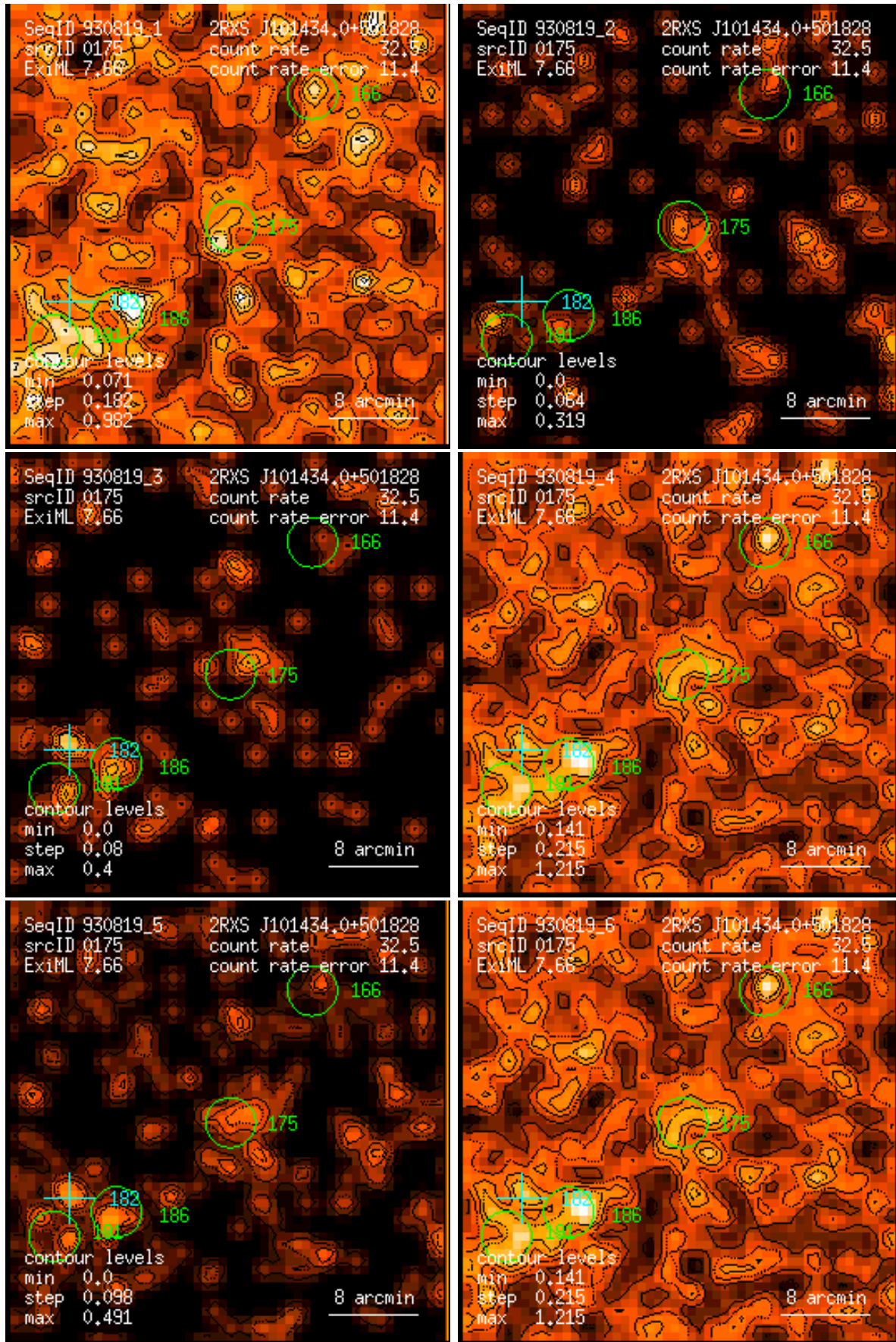
Figure 175: RASS 930819: detection 0175: band rate images, Gaussian filter: (1) PSPC channels 11 – 41, (2) 52 – 90, (3) 91 – 201, (4) 11 – 235, (5) 52 – 201, (6) 11 – 201. Broad band rates in counts/ks. Band rate contour levels in counts/ks/arcmin 2 .
