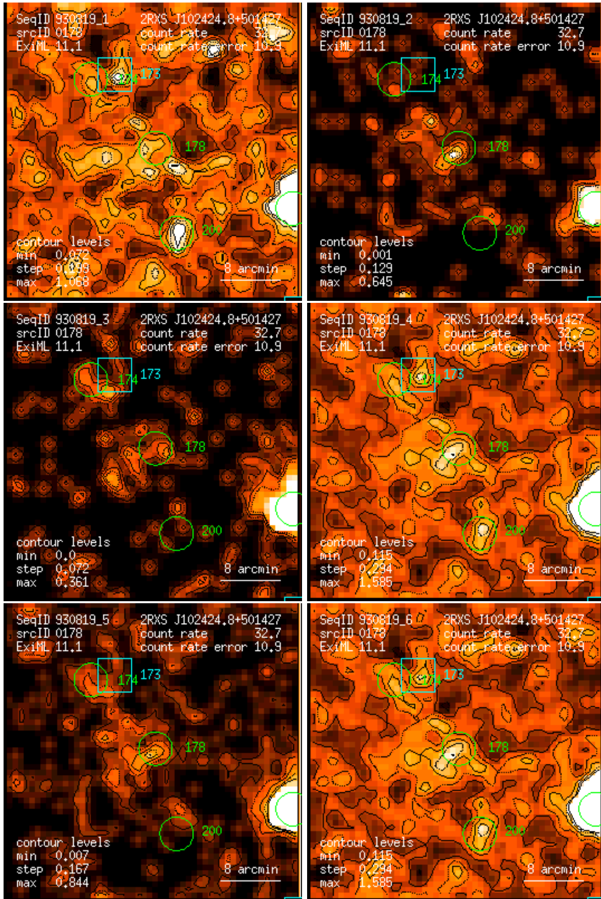
Figure 178: RASS 930819: detection 0178: band rate images, Gaussian filter: (1) PSPC channels 11 – 41, (2) 52 – 90, (3) 91 – 201, (4) 11 – 235, (5) 52 – 201, (6) 11 – 201. Broad band rates in counts/ks. Band rate contour levels in counts/ks/arcmin 2 .
