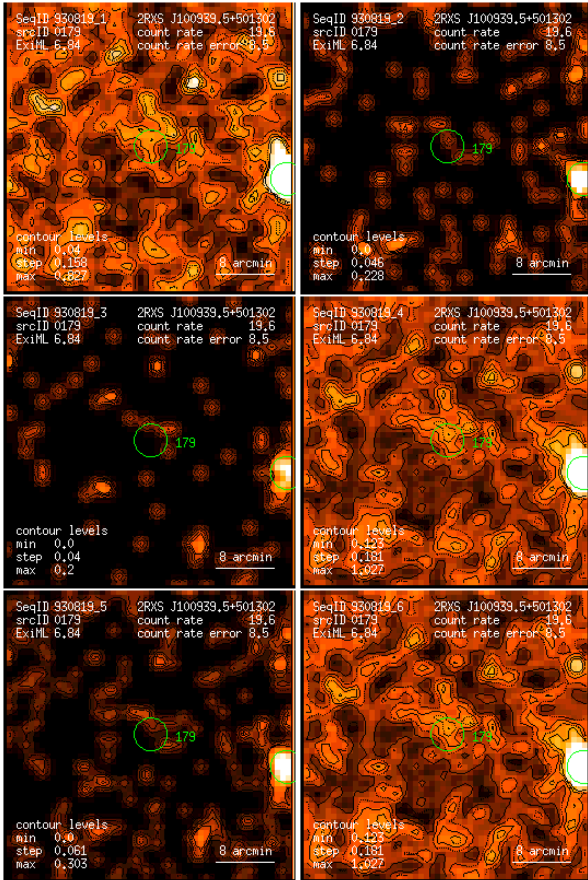
Figure 179: RASS 930819: detection 0179: band rate images, Gaussian filter: (1) PSPC channels 11 – 41, (2) 52 – 90, (3) 91 – 201, (4) 11 – 235, (5) 52 – 201, (6) 11 – 201. Broad band rates in counts/ks. Band rate contour levels in counts/ks/arcmin 2 .
