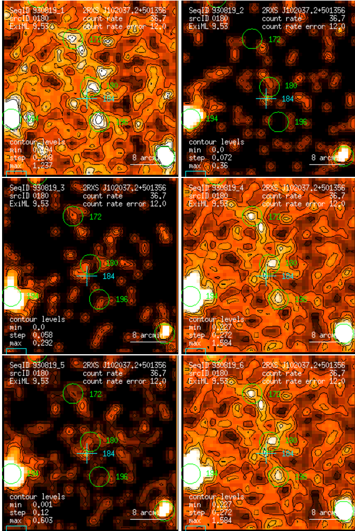
Figure 180: RASS 930819: detection 0180: band rate images, Gaussian filter: (1) PSPC channels 11 – 41, (2) 52 – 90, (3) 91 – 201, (4) 11 – 235, (5) 52 – 201, (6) 11 – 201. Broad band rates in counts/ks. Band rate contour levels in counts/ks/arcmin 2 .
