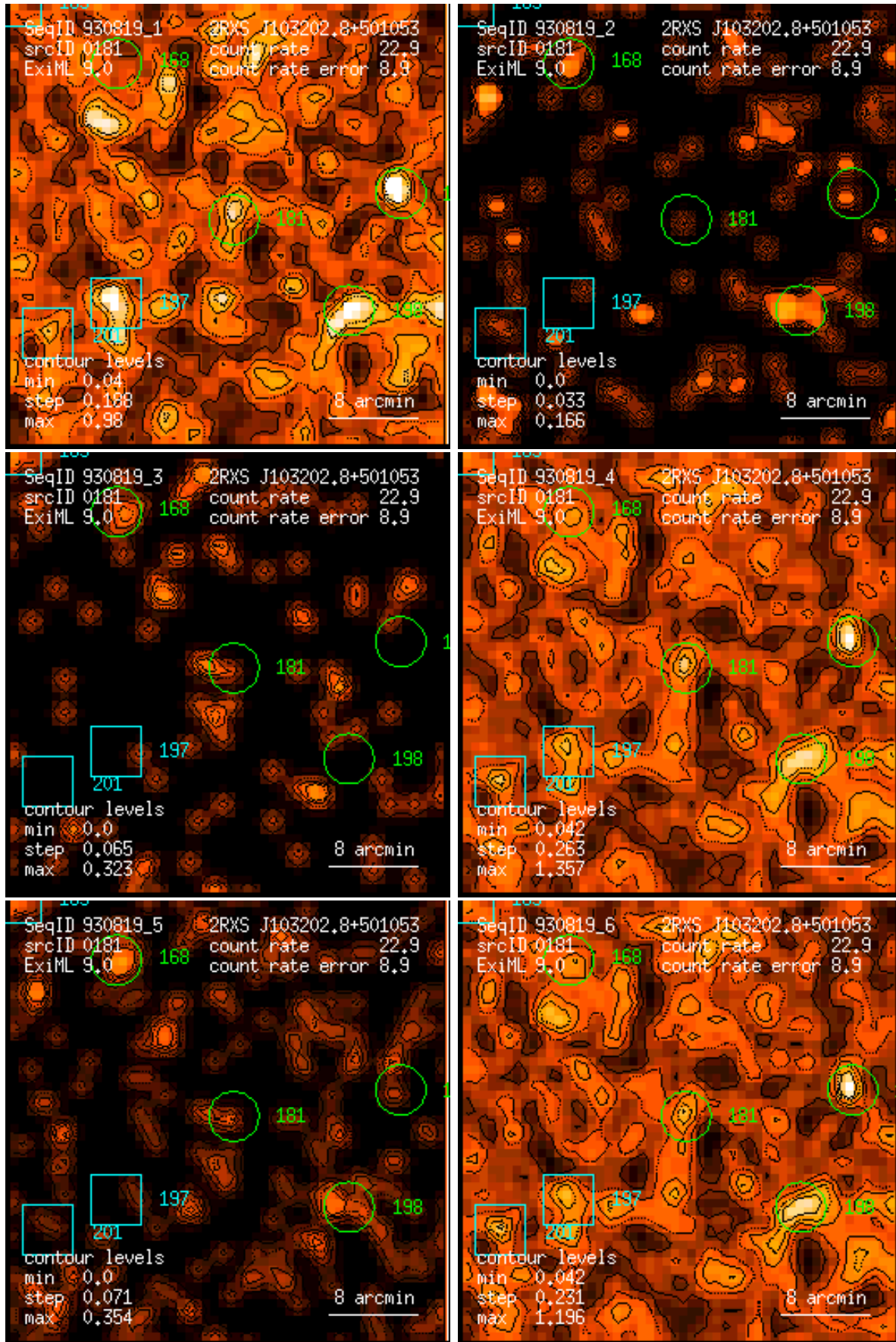
Figure 181: RASS 930819: detection 0181: band rate images, Gaussian filter: (1) PSPC channels 11 – 41, (2) 52 – 90, (3) 91 – 201, (4) 11 – 235, (5) 52 – 201, (6) 11 – 201. Broad band rates in counts/ks. Band rate contour levels in counts/ks/arcmin 2 .
