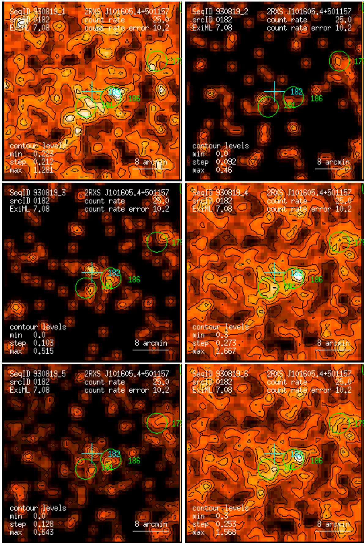
Figure 182: RASS 930819: detection 0182: band rate images, Gaussian filter: (1) PSPC channels 11 – 41, (2) 52 – 90, (3) 91 – 201, (4) 11 – 235, (5) 52 – 201, (6) 11 – 201. Broad band rates in counts/ks. Band rate contour levels in counts/ks/arcmin 2 .
