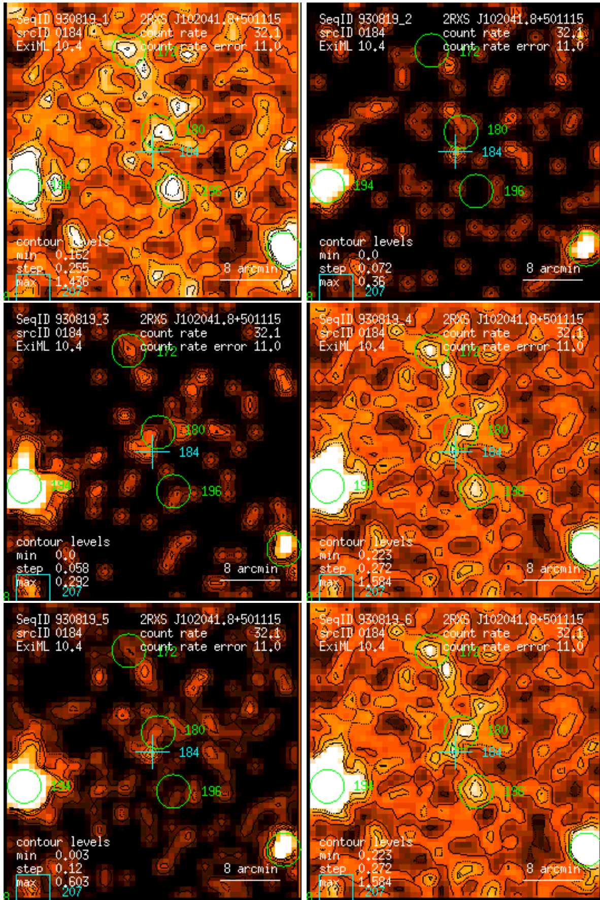
Figure 184: RASS 930819: detection 0184: band rate images, Gaussian filter: (1) PSPC channels 11 – 41, (2) 52 – 90, (3) 91 – 201, (4) 11 – 235, (5) 52 – 201, (6) 11 – 201. Broad band rates in counts/ks. Band rate contour levels in counts/ks/arcmin 2 .
