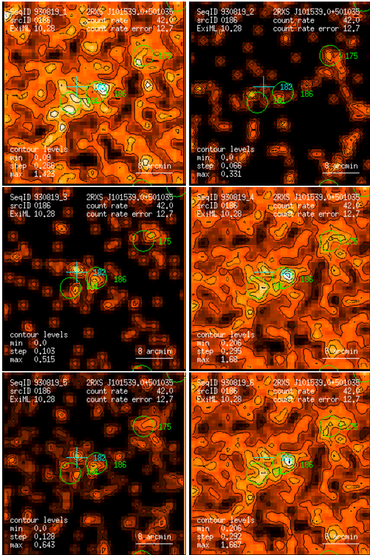
Figure 186: RASS 930819: detection 0186: band rate images, Gaussian filter: (1) PSPC channels 11 – 41, (2) 52 – 90, (3) 91 – 201, (4) 11 – 235, (5) 52 – 201, (6) 11 – 201. Broad band rates in counts/ks. Band rate contour levels in counts/ks/arcmin 2 .
