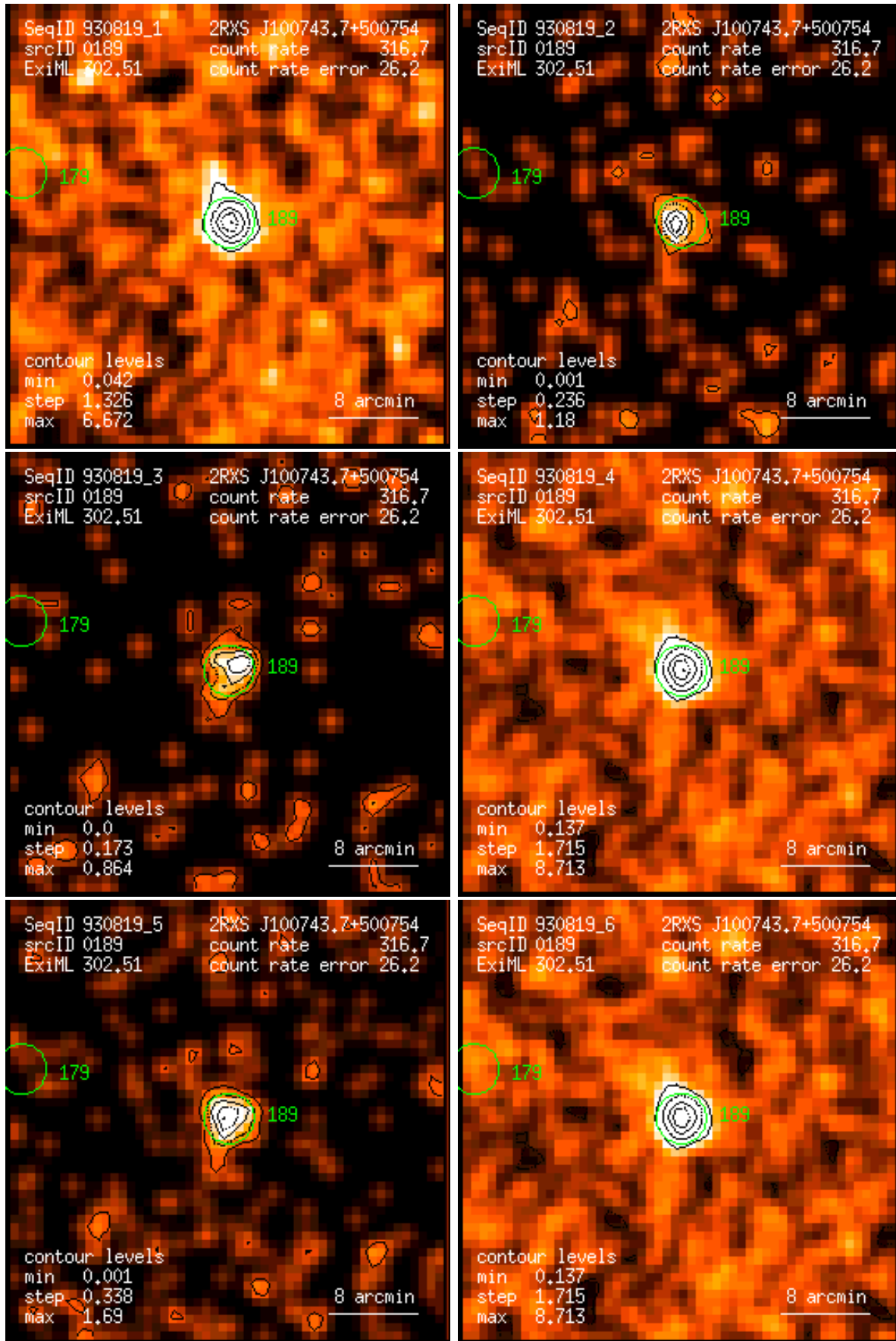
Figure 189: RASS 930819: detection 0189: band rate images, Gaussian filter: (1) PSPC channels 11 – 41, (2) 52 – 90, (3) 91 – 201, (4) 11 – 235, (5) 52 – 201, (6) 11 – 201. Broad band rates in counts/ks. Band rate contour levels in counts/ks/arcmin 2 .
