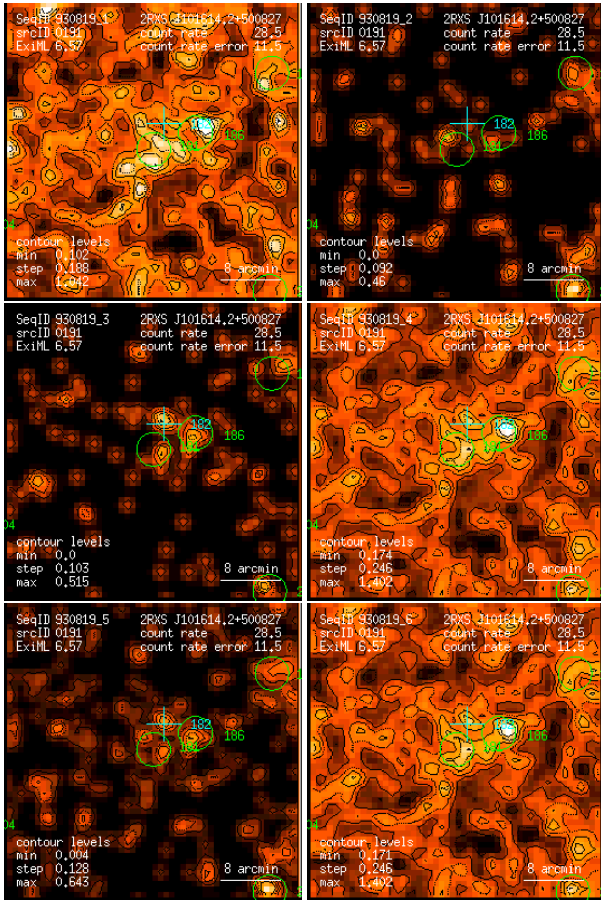
Figure 191: RASS 930819: detection 0191: band rate images, Gaussian filter: (1) PSPC channels 11 – 41, (2) 52 – 90, (3) 91 – 201, (4) 11 – 235, (5) 52 – 201, (6) 11 – 201. Broad band rates in counts/ks. Band rate contour levels in counts/ks/arcmin 2 .
