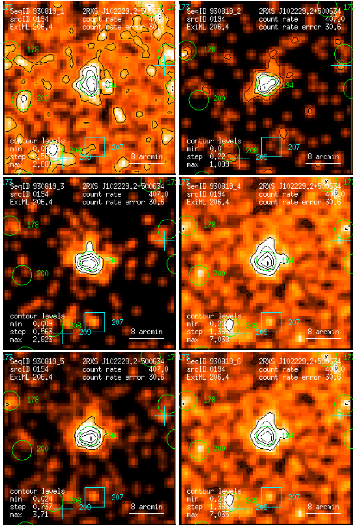
Figure 194: RASS 930819: detection 0194: band rate images, Gaussian filter: (1) PSPC channels 11 – 41, (2) 52 – 90, (3) 91 – 201, (4) 11 – 235, (5) 52 – 201, (6) 11 – 201. Broad band rates in counts/ks. Band rate contour levels in counts/ks/arcmin 2 .
