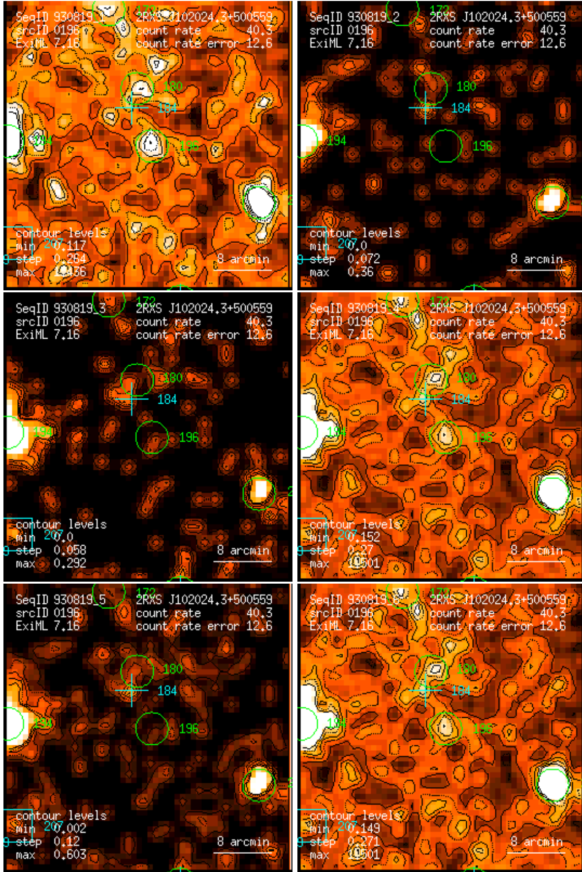
Figure 196: RASS 930819: detection 0196: band rate images, Gaussian filter: (1) PSPC channels 11 – 41, (2) 52 – 90, (3) 91 – 201, (4) 11 – 235, (5) 52 – 201, (6) 11 – 201. Broad band rates in counts/ks. Band rate contour levels in counts/ks/arcmin 2 .
