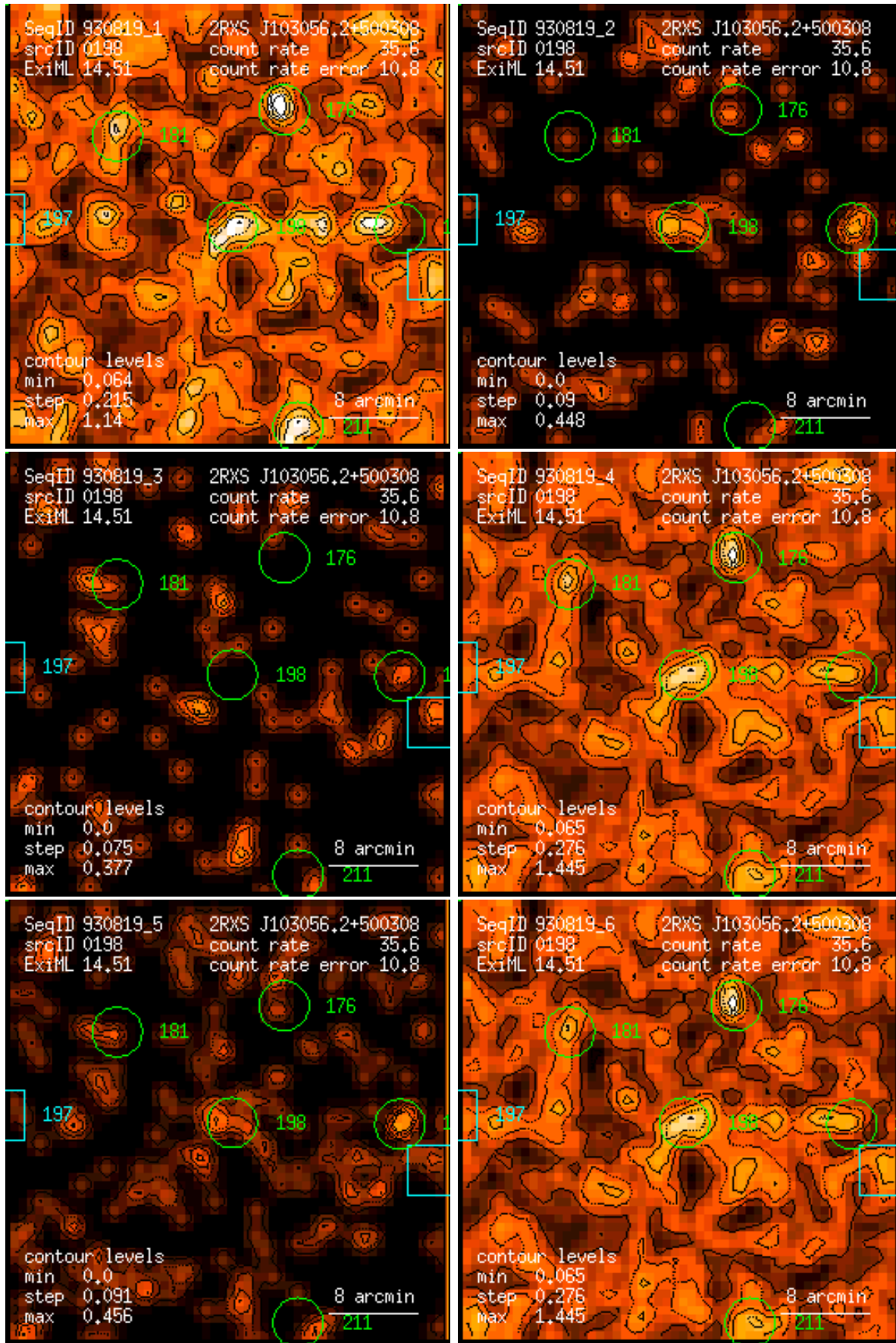
Figure 198: RASS 930819: detection 0198: band rate images, Gaussian filter: (1) PSPC channels 11 – 41, (2) 52 – 90, (3) 91 – 201, (4) 11 – 235, (5) 52 – 201, (6) 11 – 201. Broad band rates in counts/ks. Band rate contour levels in counts/ks/arcmin 2 .
