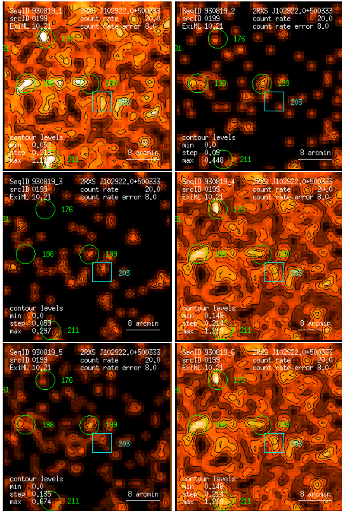
Figure 199: RASS 930819: detection 0199: band rate images, Gaussian filter: (1) PSPC channels 11 – 41, (2) 52 – 90, (3) 91 – 201, (4) 11 – 235, (5) 52 – 201, (6) 11 – 201. Broad band rates in counts/ks. Band rate contour levels in counts/ks/arcmin 2 .
