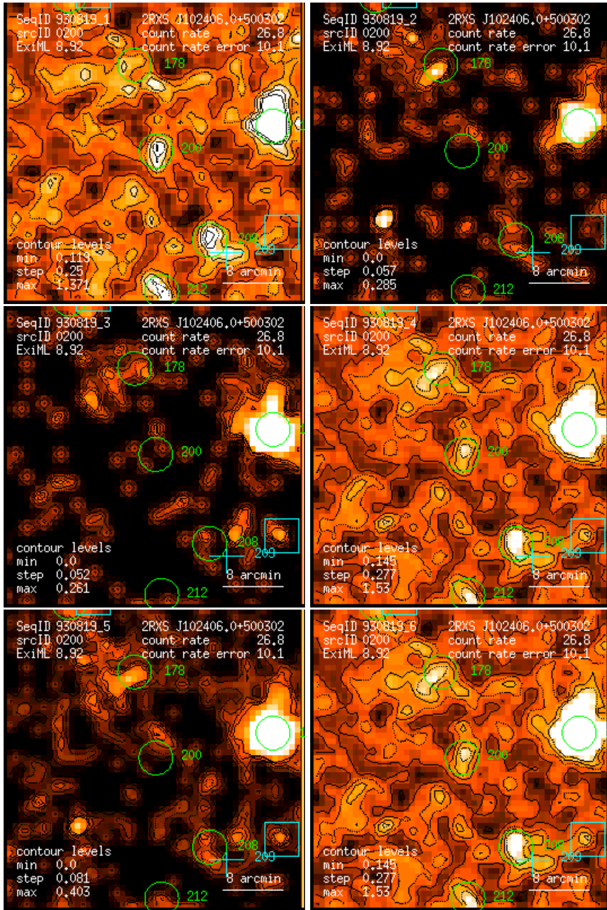
Figure 200: RASS 930819: detection 0200: band rate images, Gaussian filter: (1) PSPC channels 11 – 41, (2) 52 – 90, (3) 91 – 201, (4) 11 – 235, (5) 52 – 201, (6) 11 – 201. Broad band rates in counts/ks. Band rate contour levels in counts/ks/arcmin 2 .
