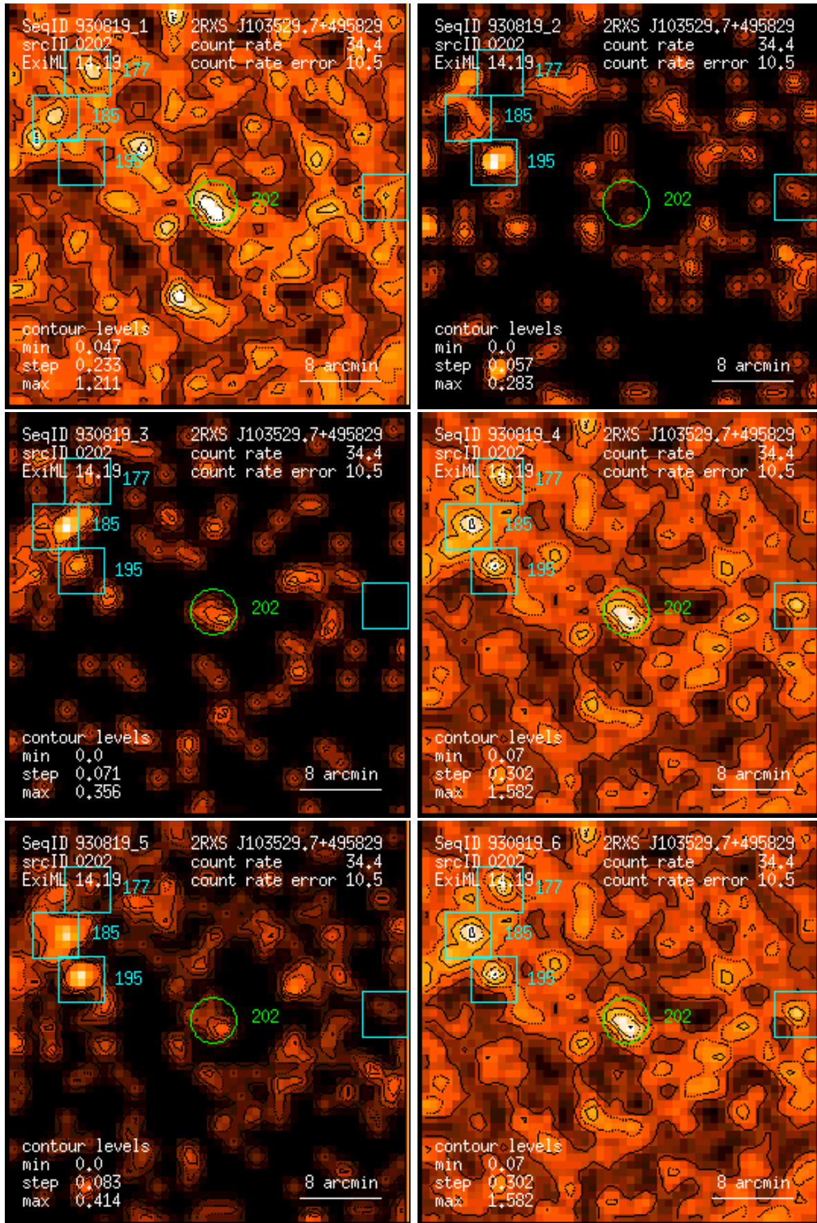
Figure 202: RASS 930819: detection 0202: band rate images, Gaussian filter: (1) PSPC channels 11 – 41, (2) 52 – 90, (3) 91 – 201, (4) 11 – 235, (5) 52 – 201, (6) 11 – 201. Broad band rates in counts/ks. Band rate contour levels in counts/ks/arcmin 2 .
